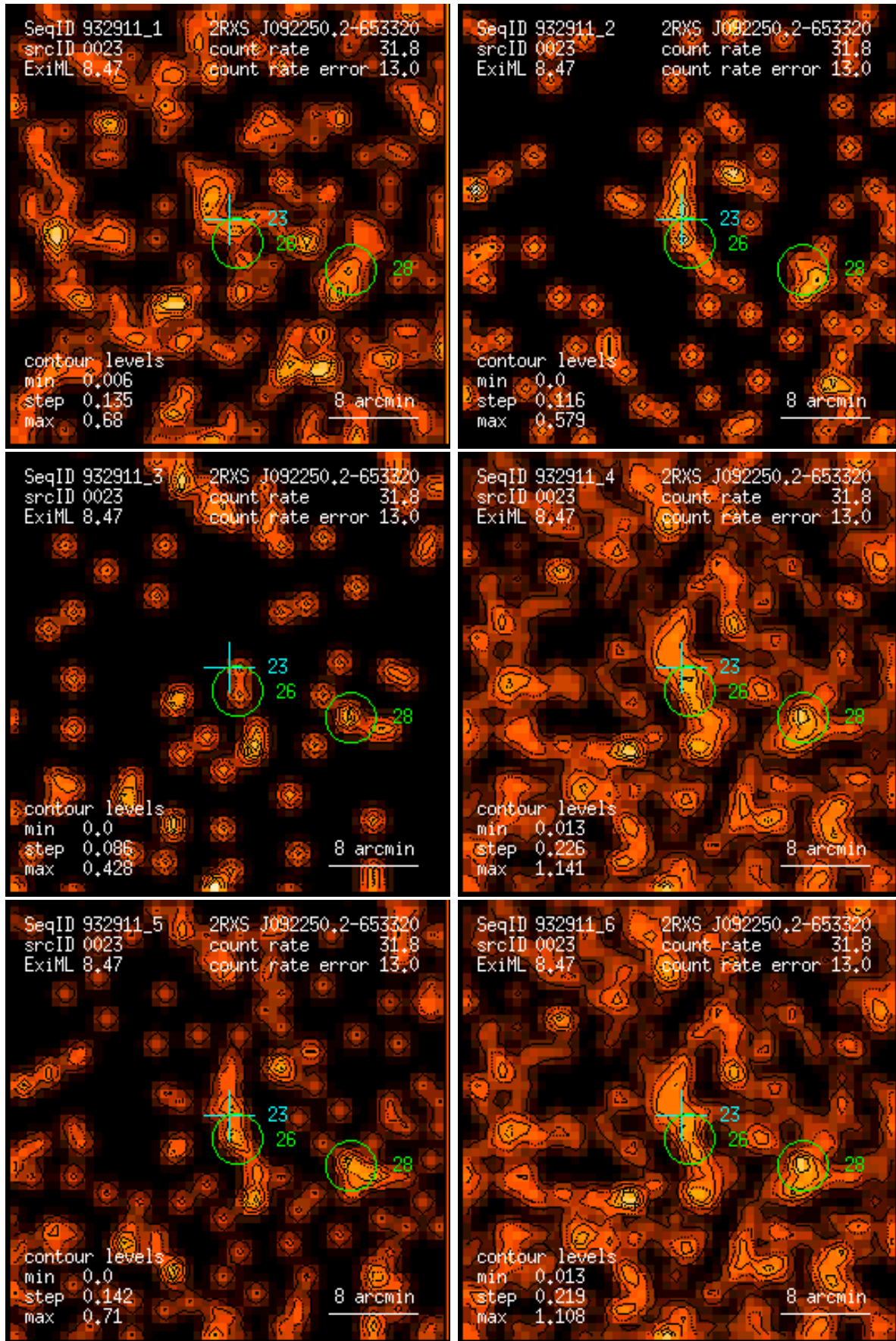
Figure 23: RASS 932911: detection 0023: band rate images, Gaussian filter: (1) PSPC channels 11 – 41, (2) 52 – 90, (3) 91 – 201, (4) 11 – 235, (5) 52 – 201, (6) 11 – 201. Broad band rates in counts/ks. Band rate contour levels in counts/ks/arcmin 2 .
