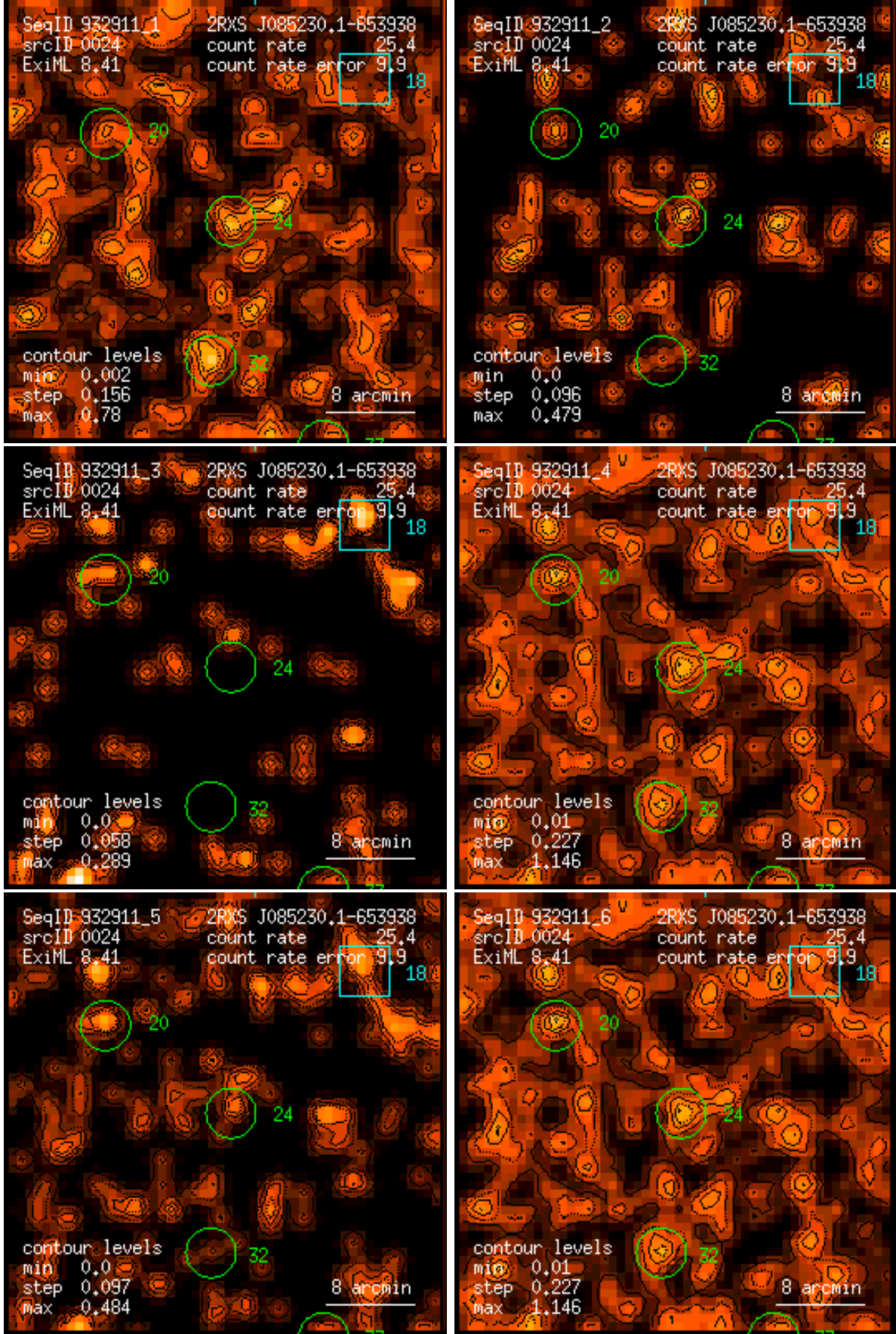
Figure 24: RASS 932911: detection 0024: band rate images, Gaussian filter: (1) PSPC channels 11 – 41, (2) 52 – 90, (3) 91 – 201, (4) 11 – 235, (5) 52 – 201, (6) 11 – 201. Broad band rates in counts/ks. Band rate contour levels in counts/ks/arcmin 2 .
