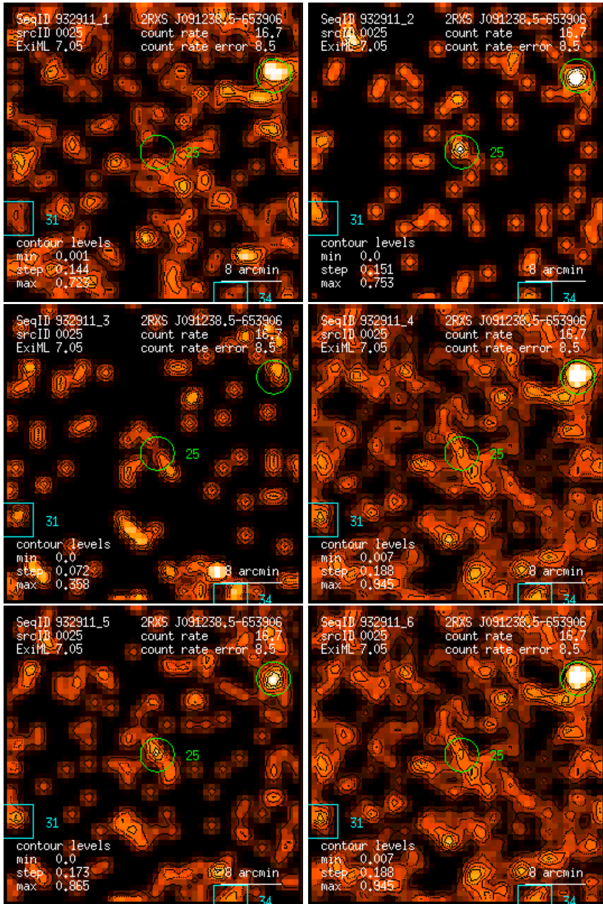
Figure 25: RASS 932911: detection 0025: band rate images, Gaussian filter: (1) PSPC channels 11 – 41, (2) 52 – 90, (3) 91 – 201, (4) 11 – 235, (5) 52 – 201, (6) 11 – 201. Broad band rates in counts/ks. Band rate contour levels in counts/ks/arcmin 2 .
