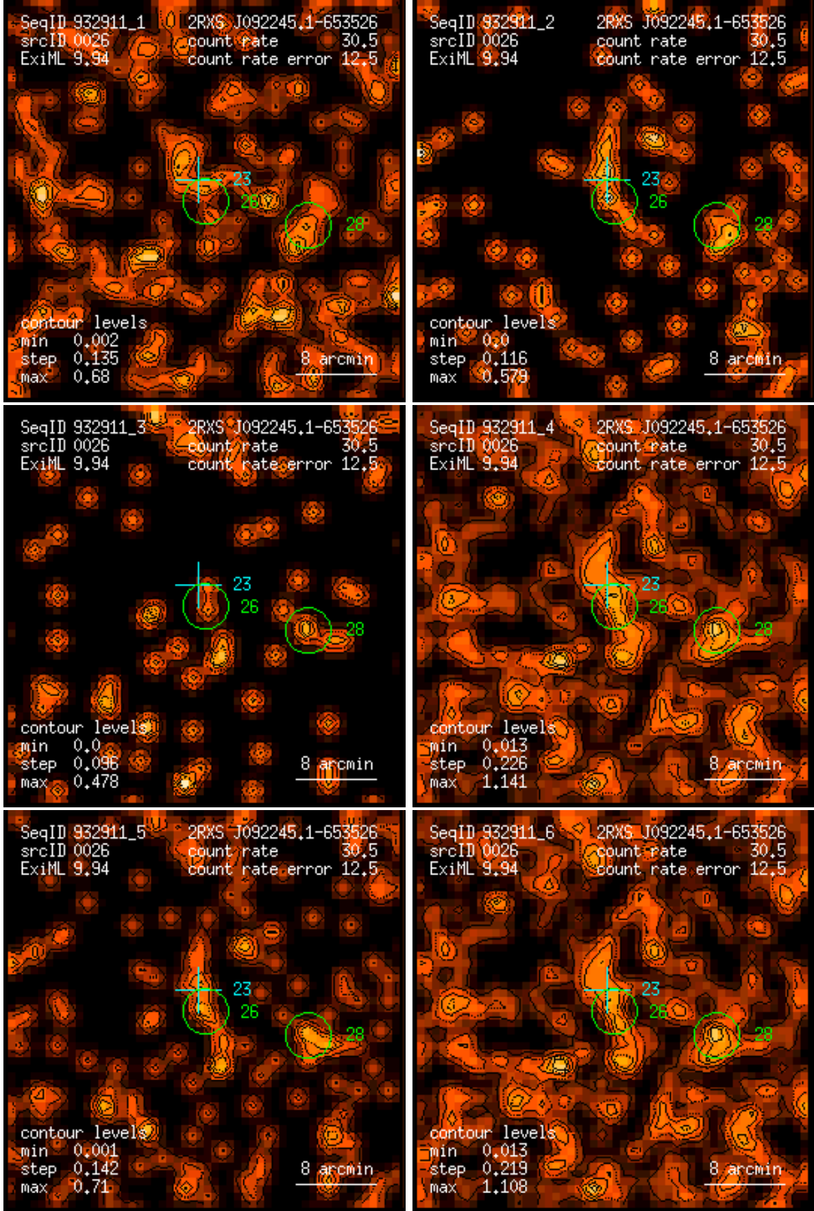
Figure 26: RASS 932911: detection 0026: band rate images, Gaussian filter: (1) PSPC channels 11 – 41, (2) 52 – 90, (3) 91 – 201, (4) 11 – 235, (5) 52 – 201, (6) 11 – 201. Broad band rates in counts/ks. Band rate contour levels in counts/ks/arcmin 2 .
