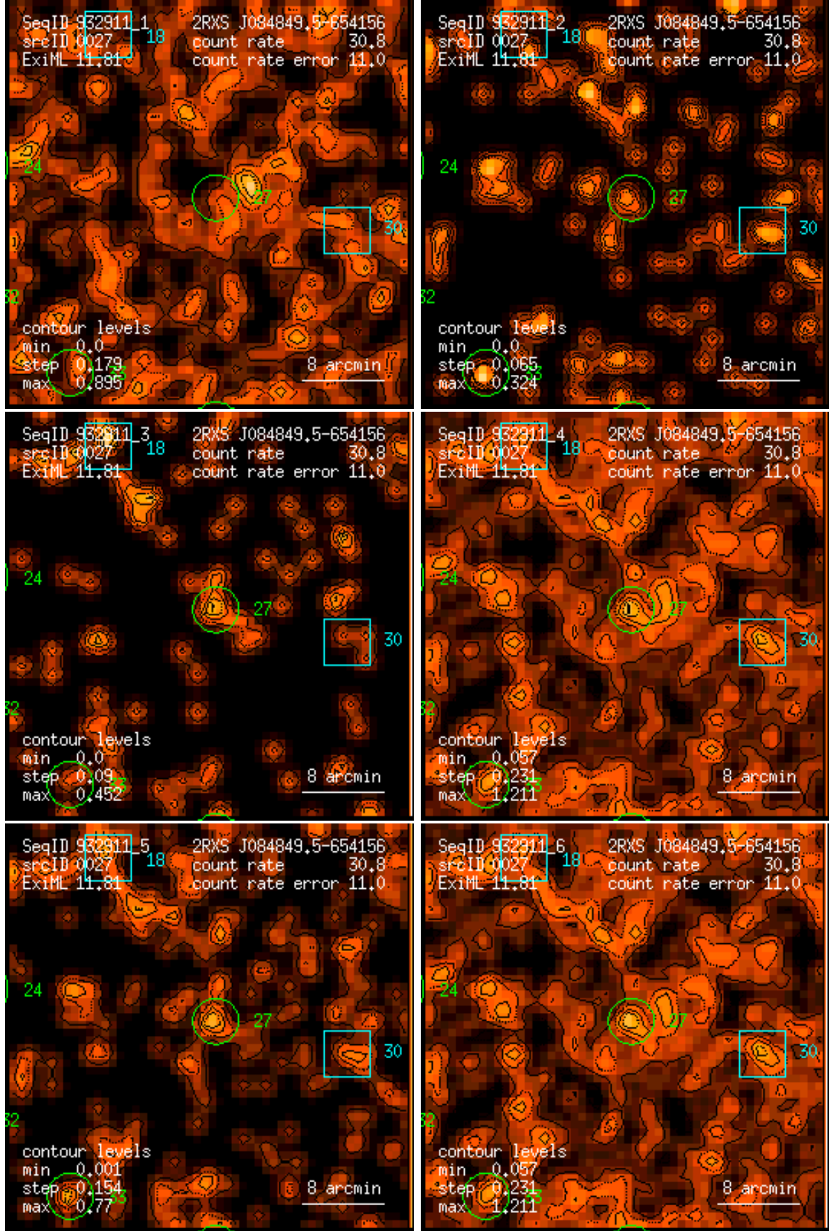
Figure 27: RASS 932911: detection 0027: band rate images, Gaussian filter: (1) PSPC channels 11 – 41, (2) 52 – 90, (3) 91 – 201, (4) 11 – 235, (5) 52 – 201, (6) 11 – 201. Broad band rates in counts/ks. Band rate contour levels in counts/ks/arcmin 2 .
