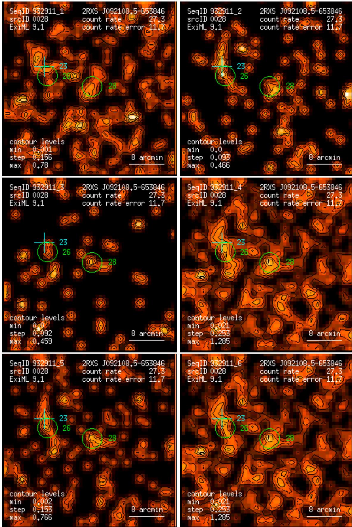
Figure 28: RASS 932911: detection 0028: band rate images, Gaussian filter: (1) PSPC channels 11 – 41, (2) 52 – 90, (3) 91 – 201, (4) 11 – 235, (5) 52 – 201, (6) 11 – 201. Broad band rates in counts/ks. Band rate contour levels in counts/ks/arcmin 2 .
