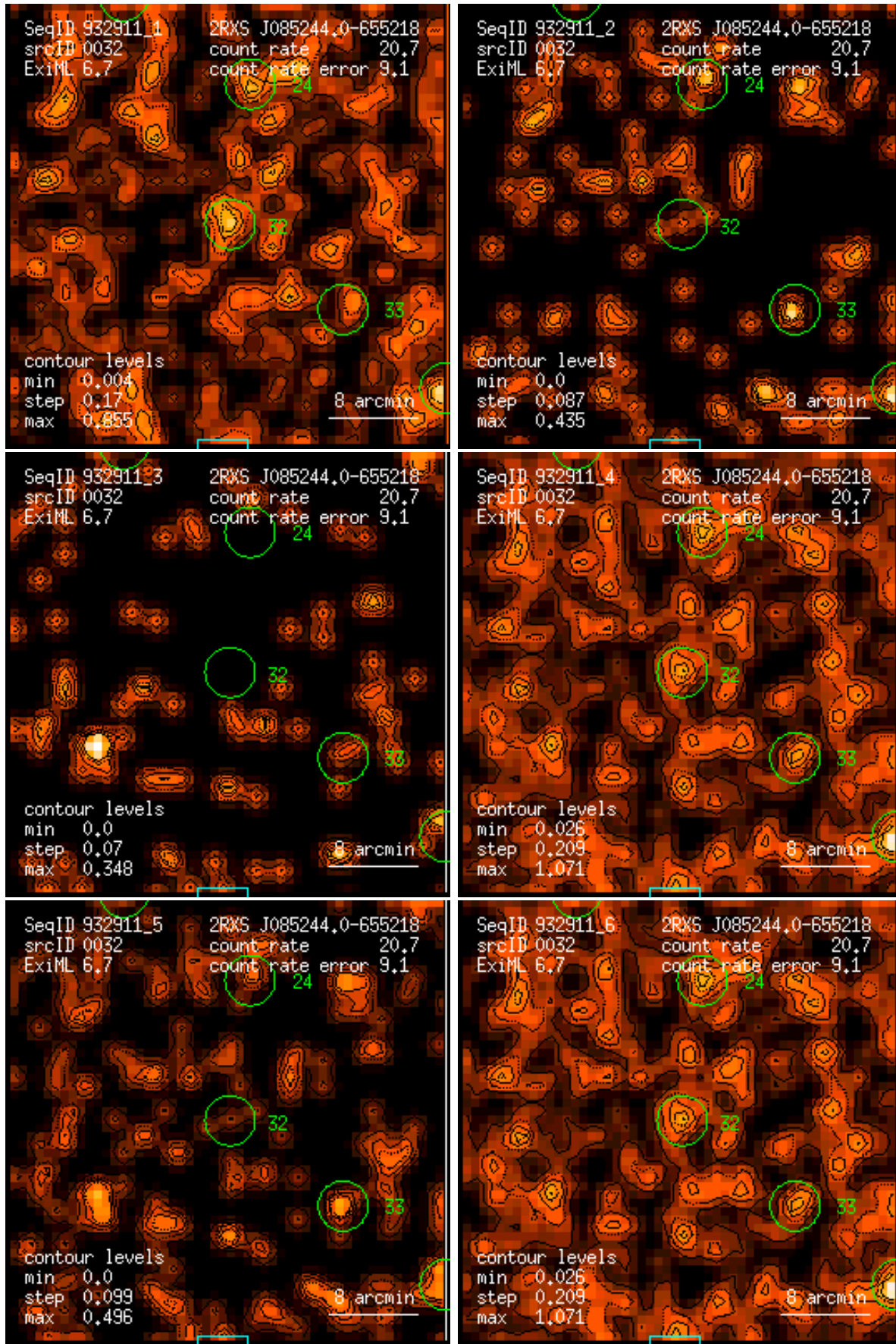
Figure 32: RASS 932911: detection 0032: band rate images, Gaussian filter: (1) PSPC channels 11 – 41, (2) 52 – 90, (3) 91 – 201, (4) 11 – 235, (5) 52 – 201, (6) 11 – 201. Broad band rates in counts/ks. Band rate contour levels in counts/ks/arcmin 2 .
