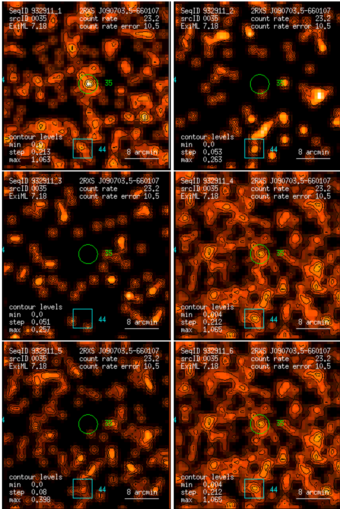
Figure 35: RASS 932911: detection 0035: band rate images, Gaussian filter: (1) PSPC channels 11 – 41, (2) 52 – 90, (3) 91 – 201, (4) 11 – 235, (5) 52 – 201, (6) 11 – 201. Broad band rates in counts/ks. Band rate contour levels in counts/ks/arcmin 2 .
