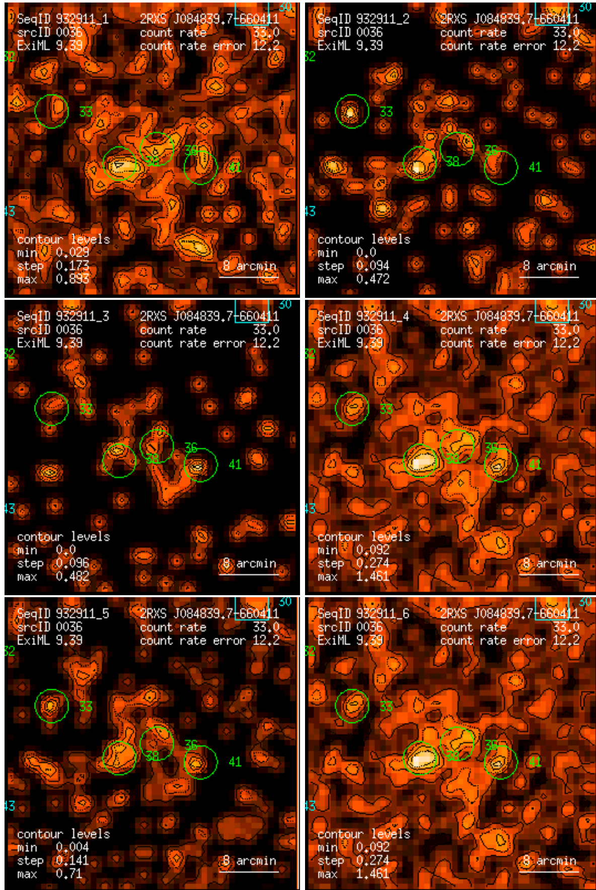
Figure 36: RASS 932911: detection 0036: band rate images, Gaussian filter: (1) PSPC channels 11 – 41, (2) 52 – 90, (3) 91 – 201, (4) 11 – 235, (5) 52 – 201, (6) 11 – 201. Broad band rates in counts/ks. Band rate contour levels in counts/ks/arcmin 2 .
