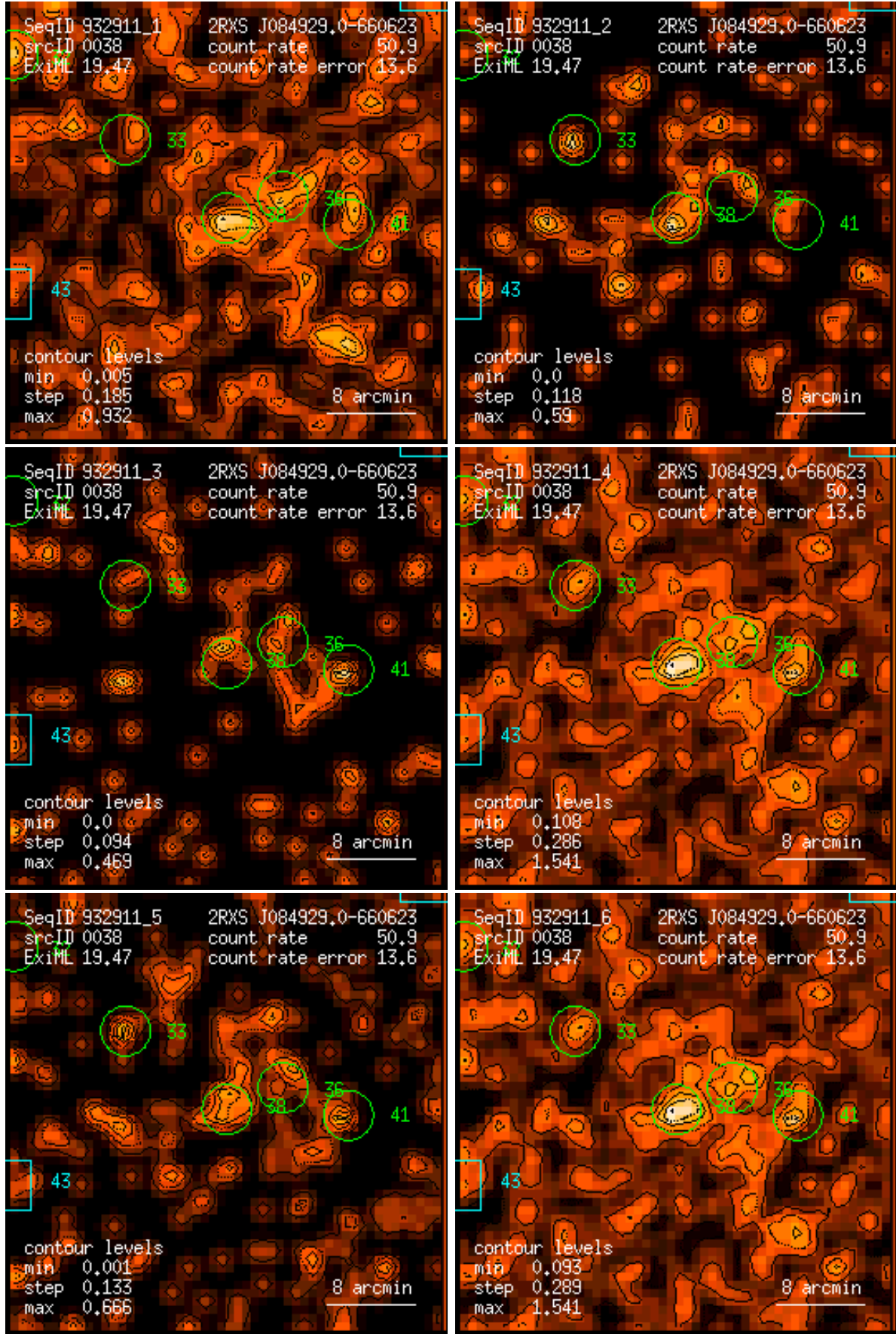
Figure 38: RASS 932911: detection 0038: band rate images, Gaussian filter: (1) PSPC channels 11 – 41, (2) 52 – 90, (3) 91 – 201, (4) 11 – 235, (5) 52 – 201, (6) 11 – 201. Broad band rates in counts/ks. Band rate contour levels in counts/ks/arcmin 2 .
