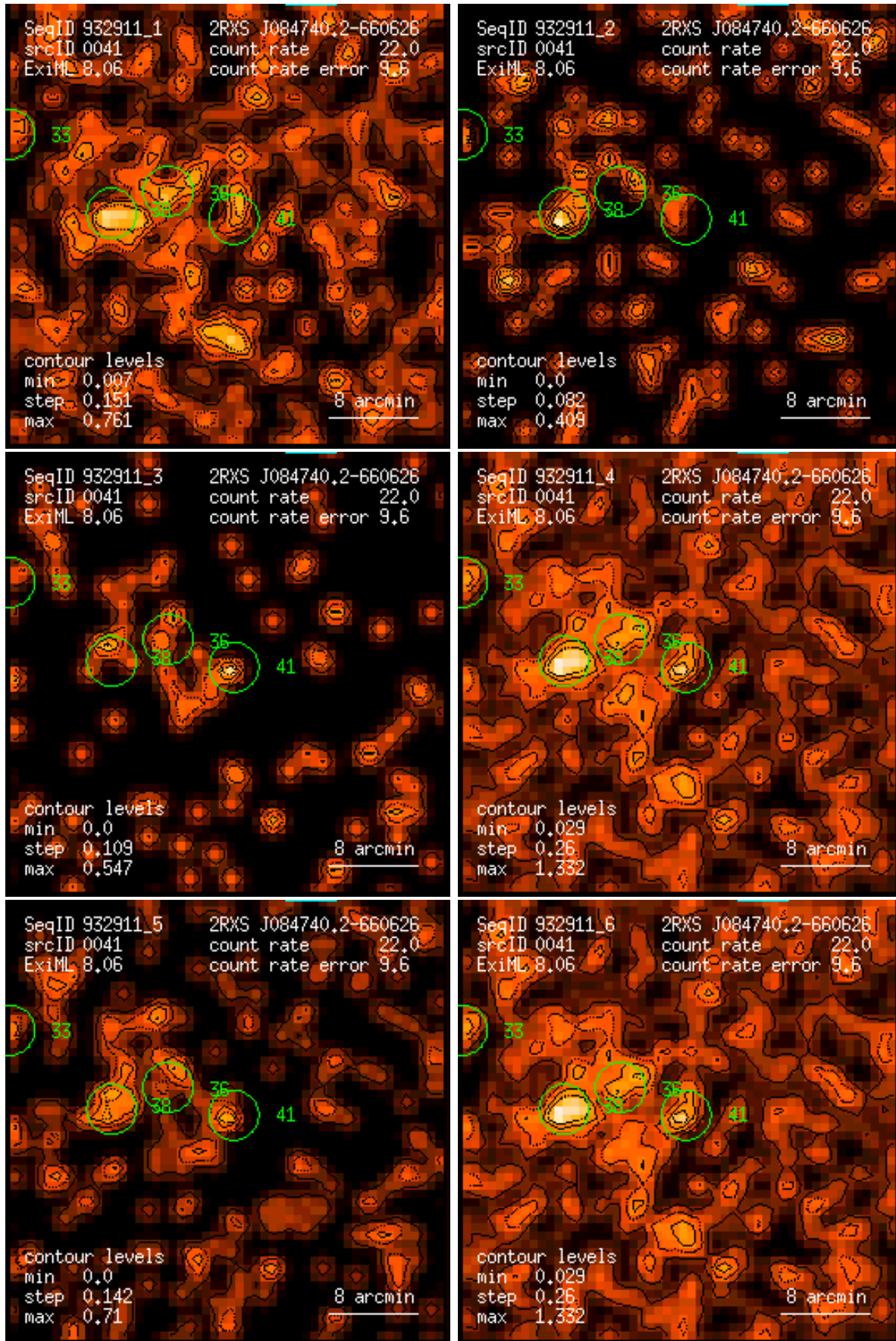
Figure 41: RASS 932911: detection 0041: band rate images, Gaussian filter: (1) PSPC channels 11 – 41, (2) 52 – 90, (3) 91 – 201, (4) 11 – 235, (5) 52 – 201, (6) 11 – 201. Broad band rates in counts/ks. Band rate contour levels in counts/ks/arcmin 2 .
