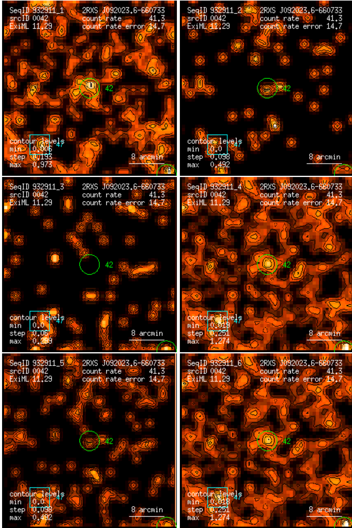
Figure 42: RASS 932911: detection 0042: band rate images, Gaussian filter: (1) PSPC channels 11 – 41, (2) 52 – 90, (3) 91 – 201, (4) 11 – 235, (5) 52 – 201, (6) 11 – 201. Broad band rates in counts/ks. Band rate contour levels in counts/ks/arcmin 2 .
