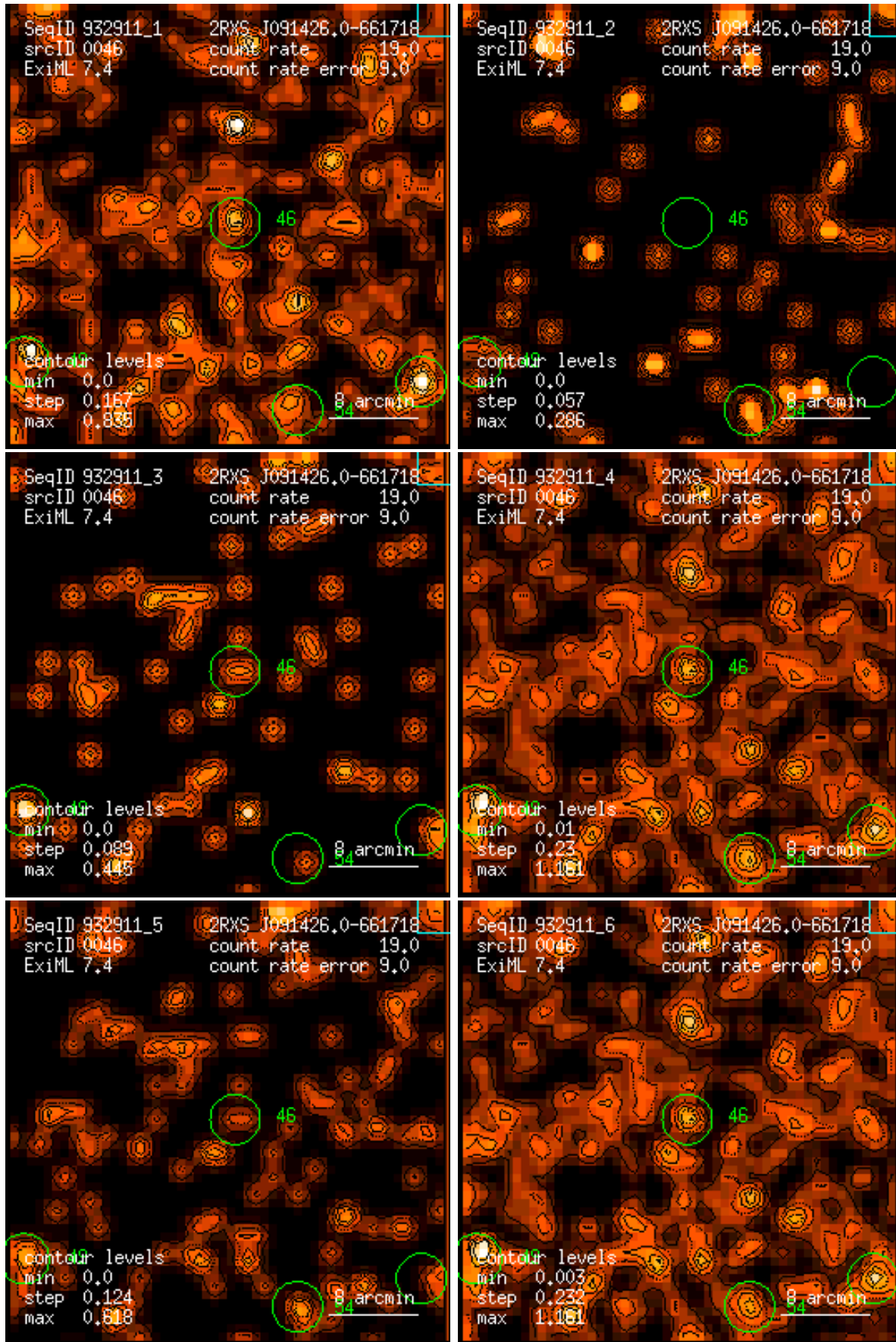
Figure 46: RASS 932911: detection 0046: band rate images, Gaussian filter: (1) PSPC channels 11 – 41, (2) 52 – 90, (3) 91 – 201, (4) 11 – 235, (5) 52 – 201, (6) 11 – 201. Broad band rates in counts/ks. Band rate contour levels in counts/ks/arcmin 2 .
