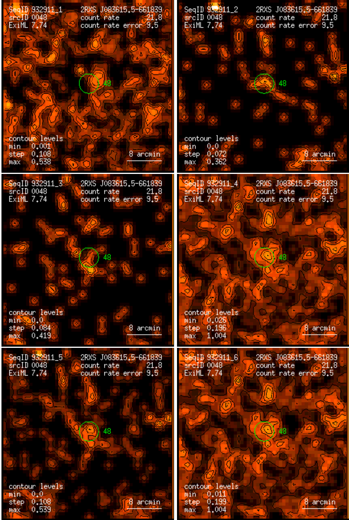
Figure 48: RASS 932911: detection 0048: band rate images, Gaussian filter: (1) PSPC channels 11 – 41, (2) 52 – 90, (3) 91 – 201, (4) 11 – 235, (5) 52 – 201, (6) 11 – 201. Broad band rates in counts/ks. Band rate contour levels in counts/ks/arcmin 2 .
