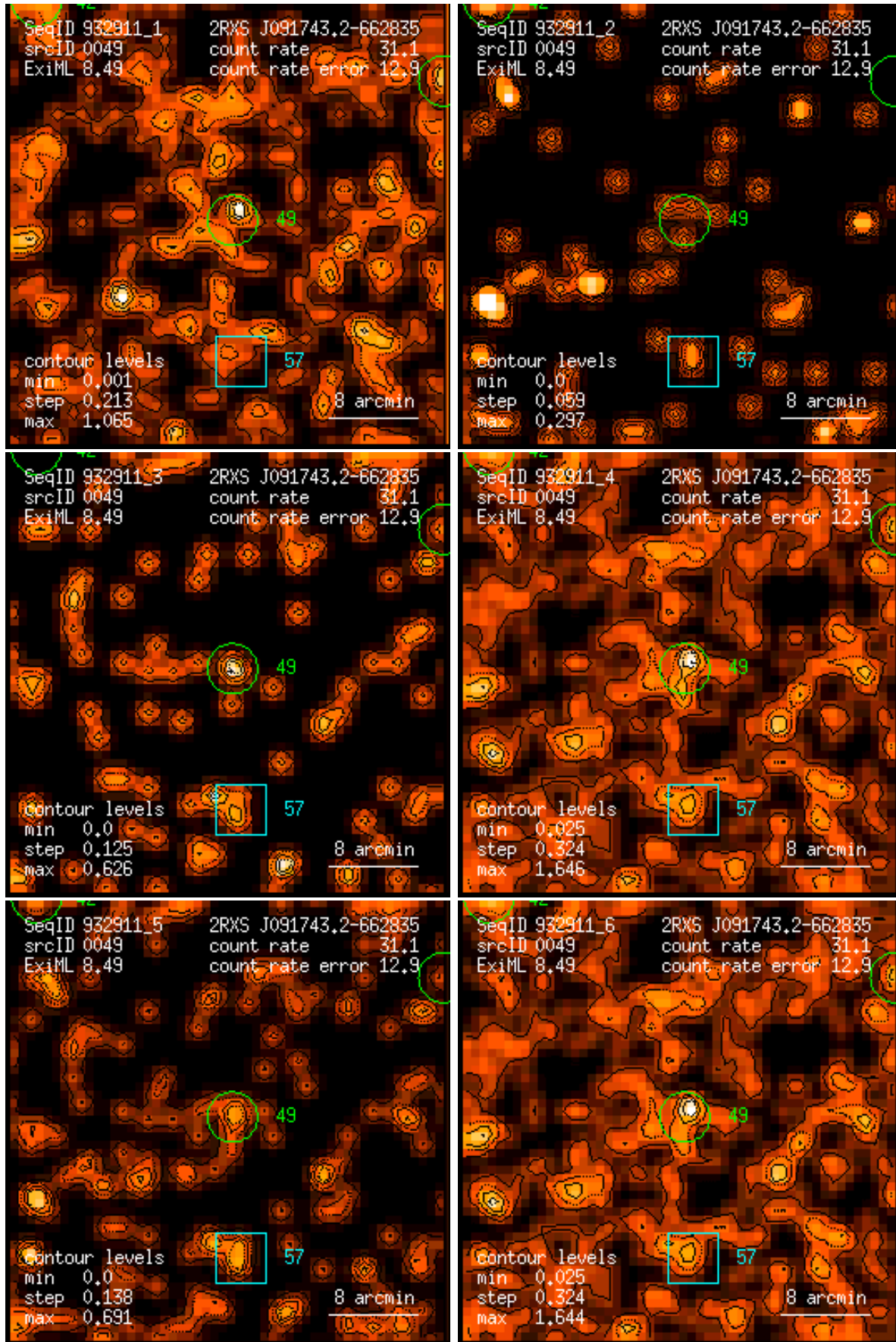
Figure 49: RASS 932911: detection 0049: band rate images, Gaussian filter: (1) PSPC channels 11 – 41, (2) 52 – 90, (3) 91 – 201, (4) 11 – 235, (5) 52 – 201, (6) 11 – 201. Broad band rates in counts/ks. Band rate contour levels in counts/ks/arcmin 2 .
