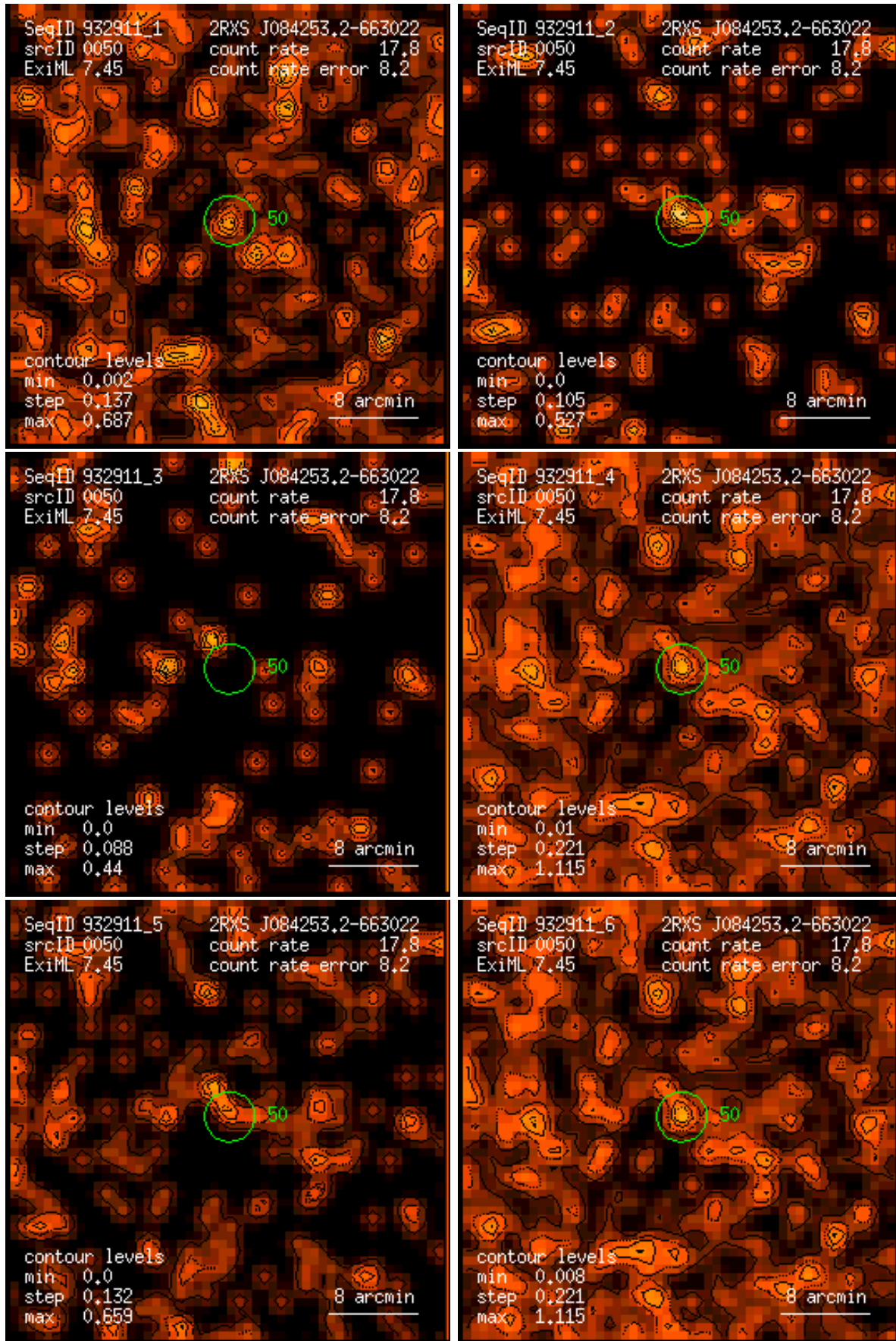
Figure 50: RASS 932911: detection 0050: band rate images, Gaussian filter: (1) PSPC channels 11 – 41, (2) 52 – 90, (3) 91 – 201, (4) 11 – 235, (5) 52 – 201, (6) 11 – 201. Broad band rates in counts/ks. Band rate contour levels in counts/ks/arcmin 2 .
