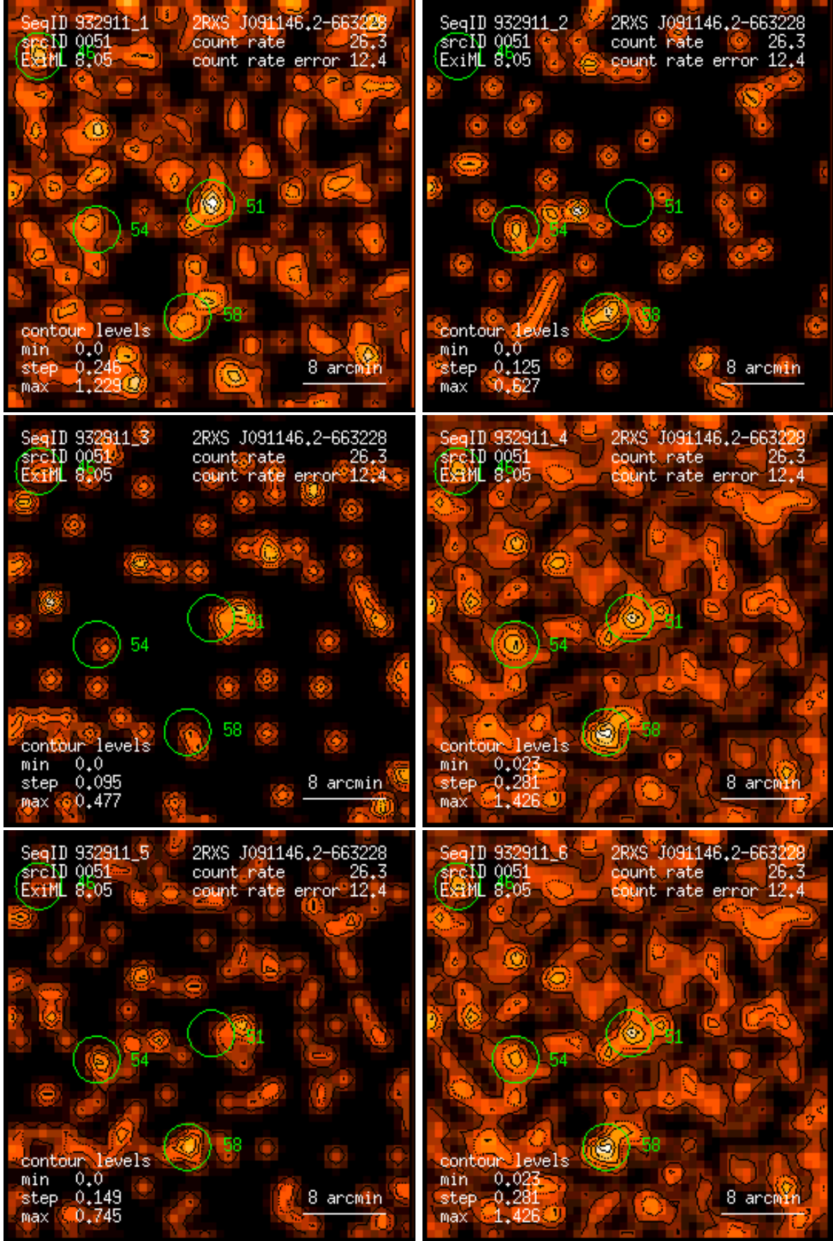
Figure 51: RASS 932911: detection 0051: band rate images, Gaussian filter: (1) PSPC channels 11 – 41, (2) 52 – 90, (3) 91 – 201, (4) 11 – 235, (5) 52 – 201, (6) 11 – 201. Broad band rates in counts/ks. Band rate contour levels in counts/ks/arcmin 2 .
