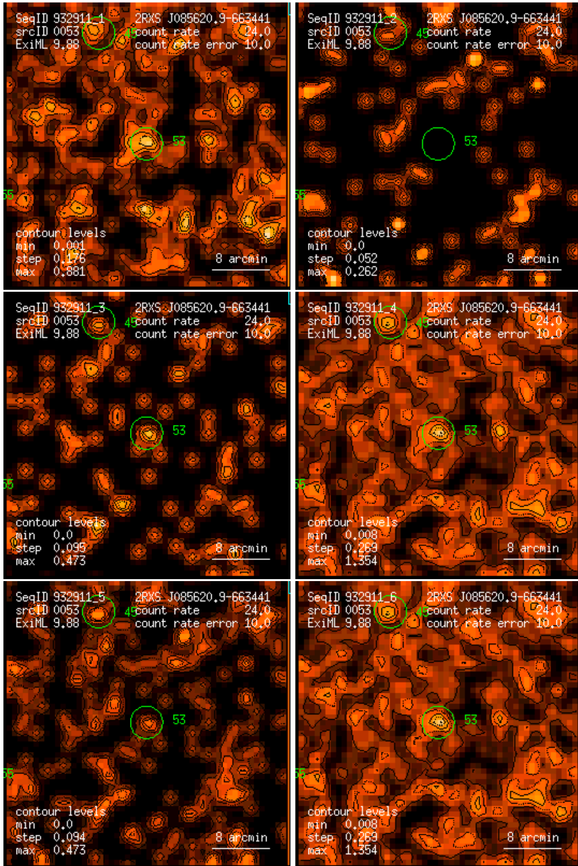
Figure 53: RASS 932911: detection 0053: band rate images, Gaussian filter: (1) PSPC channels 11 – 41, (2) 52 – 90, (3) 91 – 201, (4) 11 – 235, (5) 52 – 201, (6) 11 – 201. Broad band rates in counts/ks. Band rate contour levels in counts/ks/arcmin 2 .
