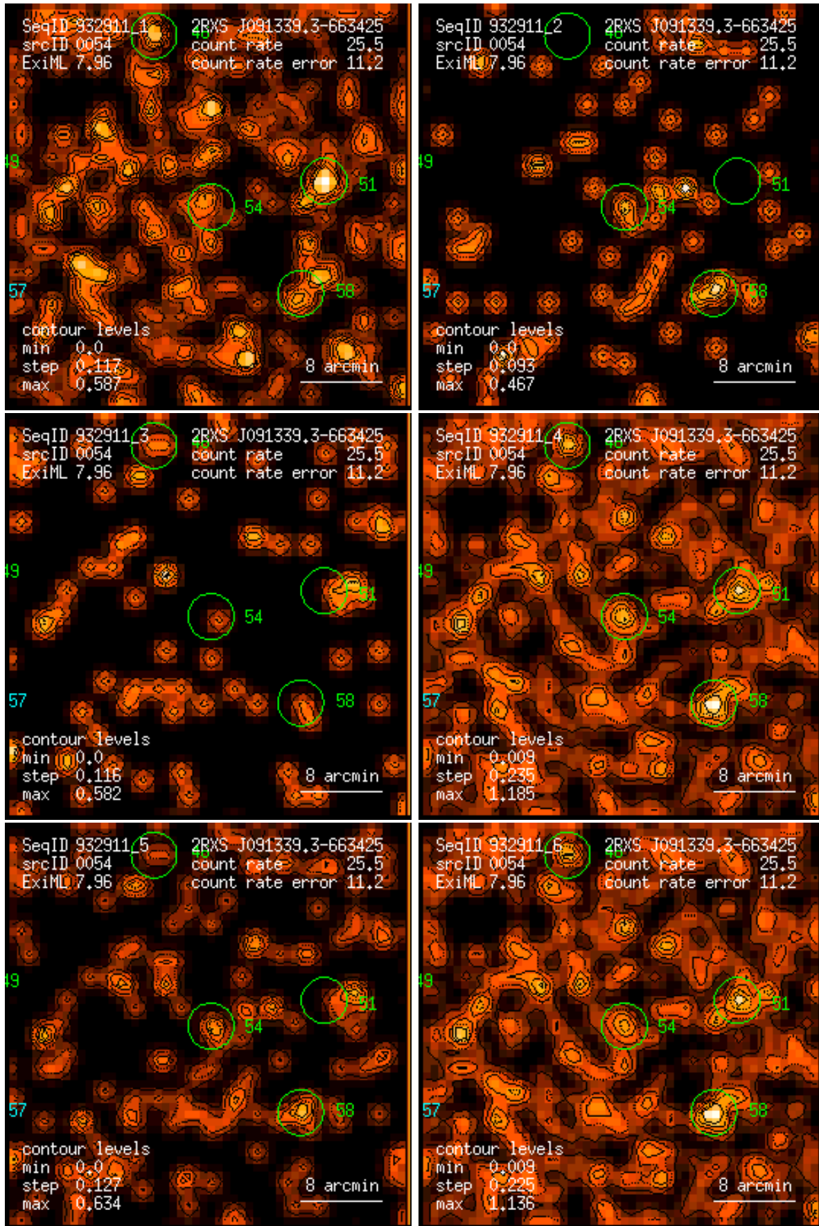
Figure 54: RASS 932911: detection 0054: band rate images, Gaussian filter: (1) PSPC channels 11 – 41, (2) 52 – 90, (3) 91 – 201, (4) 11 – 235, (5) 52 – 201, (6) 11 – 201. Broad band rates in counts/ks. Band rate contour levels in counts/ks/arcmin 2 .
