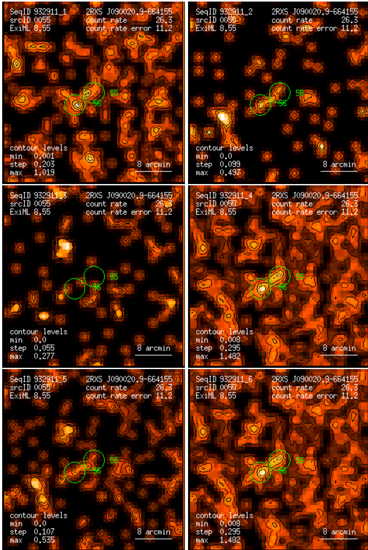
Figure 55: RASS 932911: detection 0055: band rate images, Gaussian filter: (1) PSPC channels 11 – 41, (2) 52 – 90, (3) 91 – 201, (4) 11 – 235, (5) 52 – 201, (6) 11 – 201. Broad band rates in counts/ks. Band rate contour levels in counts/ks/arcmin 2 .
