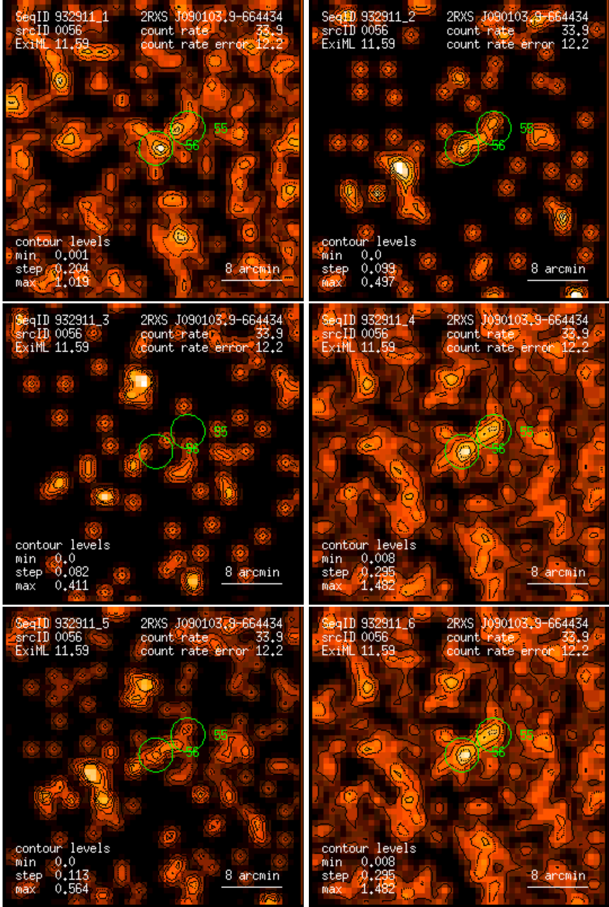
Figure 56: RASS 932911: detection 0056: band rate images, Gaussian filter: (1) PSPC channels 11 – 41, (2) 52 – 90, (3) 91 – 201, (4) 11 – 235, (5) 52 – 201, (6) 11 – 201. Broad band rates in counts/ks. Band rate contour levels in counts/ks/arcmin 2 .
