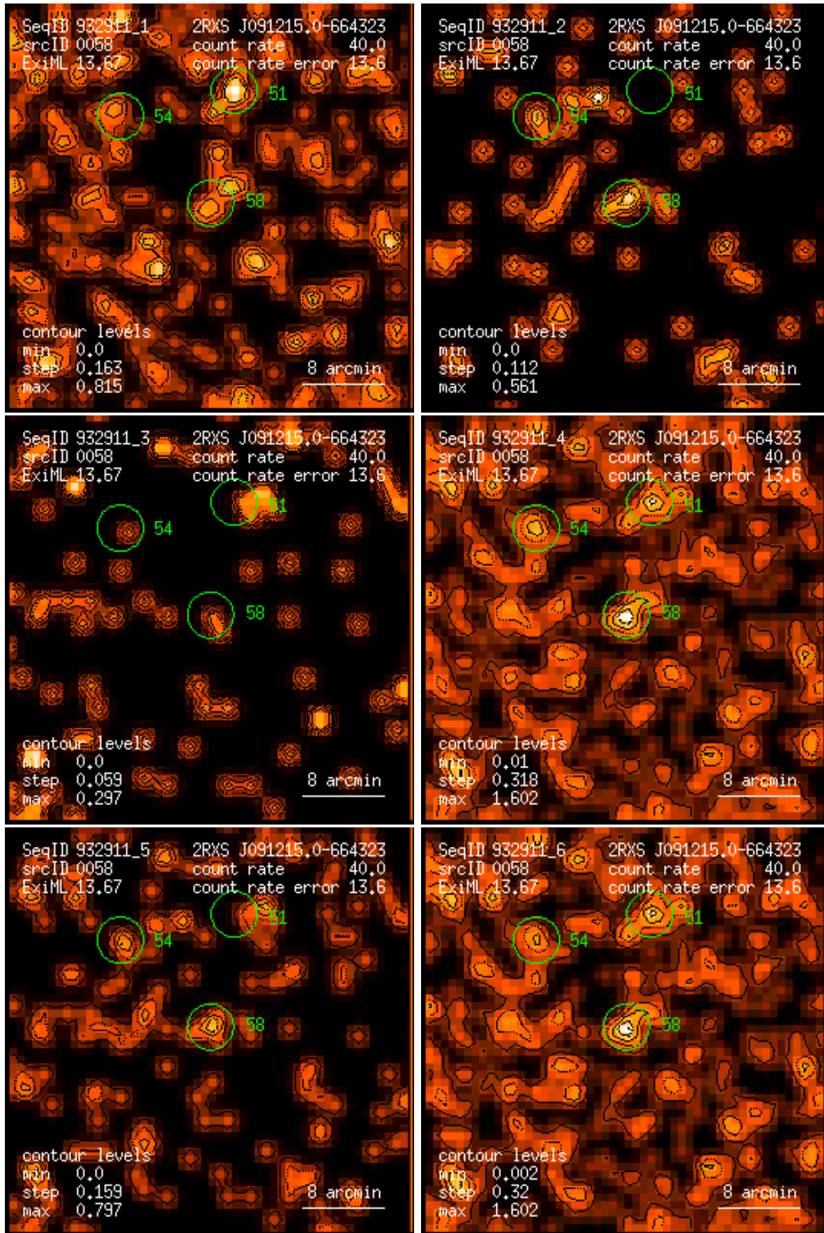
Figure 58: RASS 932911: detection 0058: band rate images, Gaussian filter: (1) PSPC channels 11 – 41, (2) 52 – 90, (3) 91 – 201, (4) 11 – 235, (5) 52 – 201, (6) 11 – 201. Broad band rates in counts/ks. Band rate contour levels in counts/ks/arcmin 2 .
