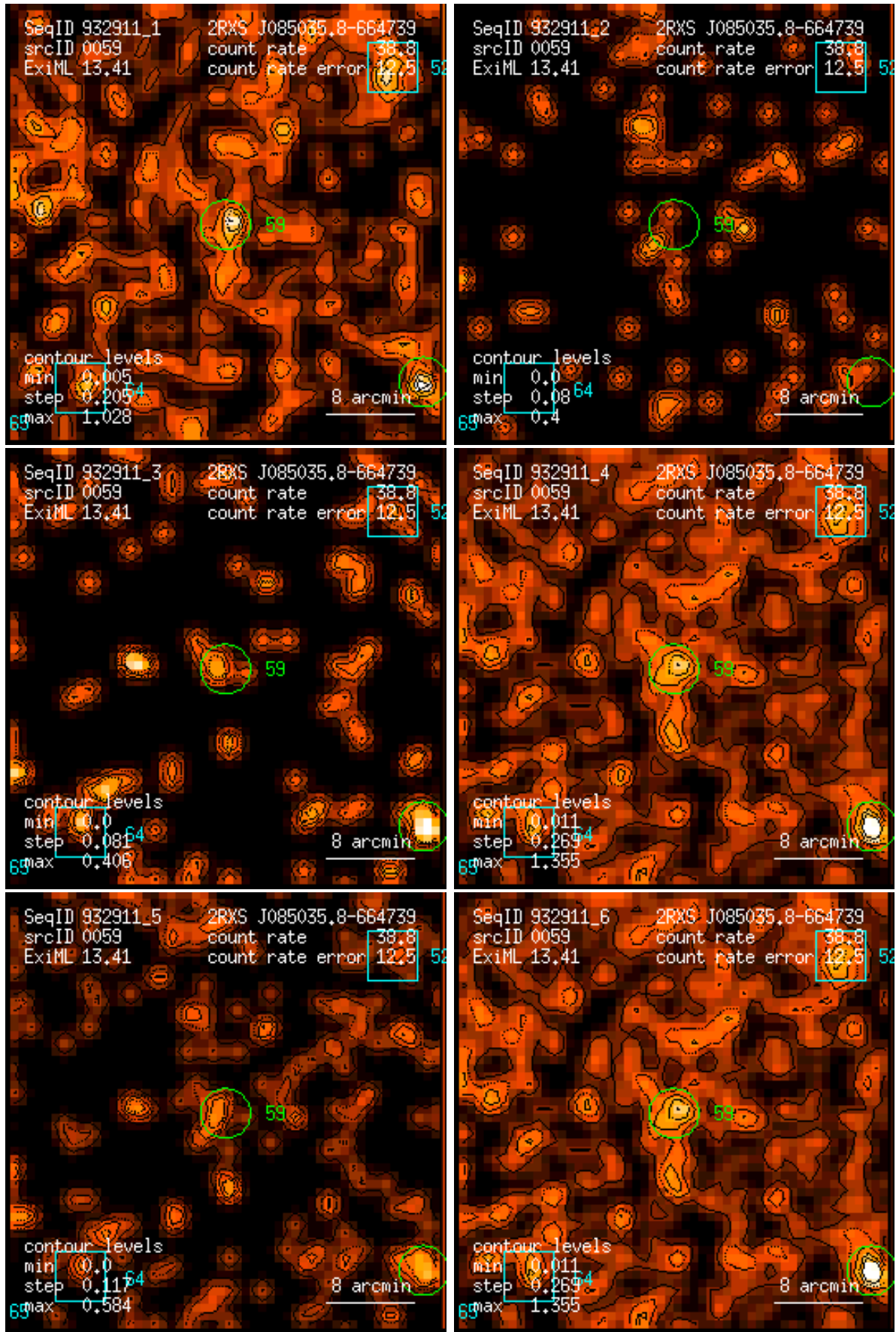
Figure 59: RASS 932911: detection 0059: band rate images, Gaussian filter: (1) PSPC channels 11 – 41, (2) 52 – 90, (3) 91 – 201, (4) 11 – 235, (5) 52 – 201, (6) 11 – 201. Broad band rates in counts/ks. Band rate contour levels in counts/ks/arcmin 2 .
