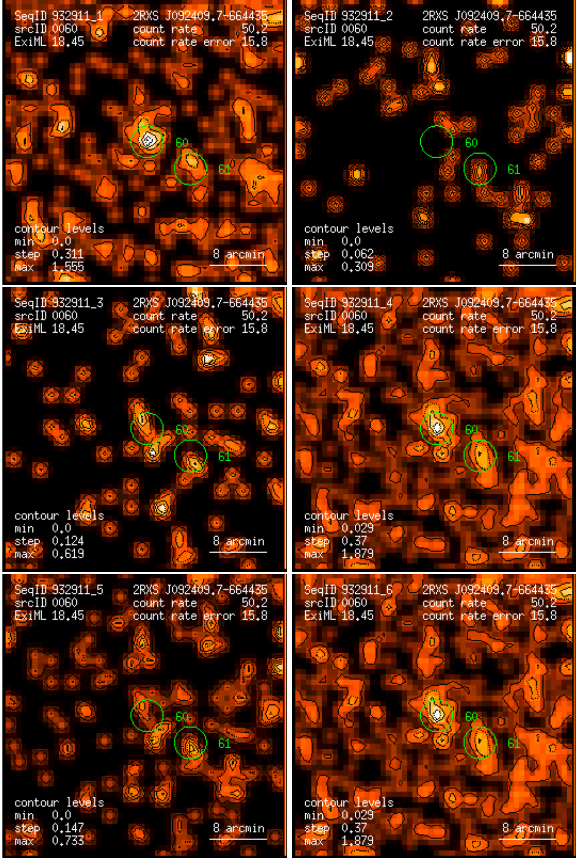
Figure 60: RASS 932911: detection 0060: band rate images, Gaussian filter: (1) PSPC channels 11 – 41, (2) 52 – 90, (3) 91 – 201, (4) 11 – 235, (5) 52 – 201, (6) 11 – 201. Broad band rates in counts/ks. Band rate contour levels in counts/ks/arcmin 2 .
