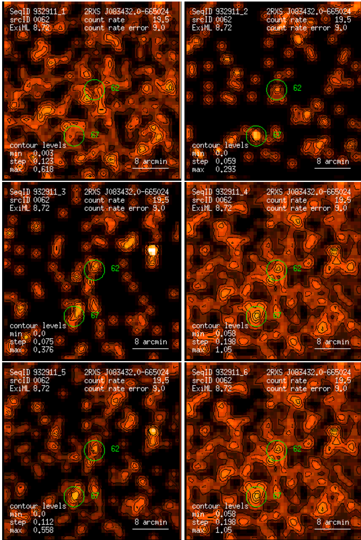
Figure 62: RASS 932911: detection 0062: band rate images, Gaussian filter: (1) PSPC channels 11 – 41, (2) 52 – 90, (3) 91 – 201, (4) 11 – 235, (5) 52 – 201, (6) 11 – 201. Broad band rates in counts/ks. Band rate contour levels in counts/ks/arcmin 2 .
