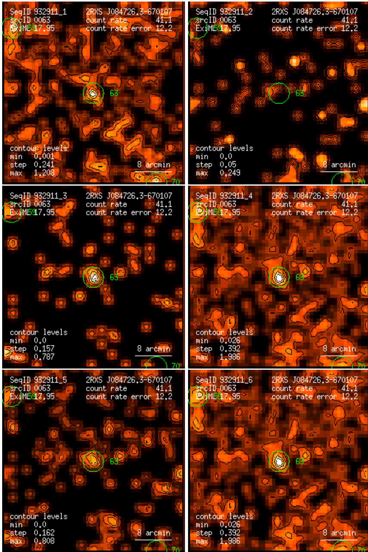
Figure 63: RASS 932911: detection 0063: band rate images, Gaussian filter: (1) PSPC channels 11 – 41, (2) 52 – 90, (3) 91 – 201, (4) 11 – 235, (5) 52 – 201, (6) 11 – 201. Broad band rates in counts/ks. Band rate contour levels in counts/ks/arcmin 2 .
