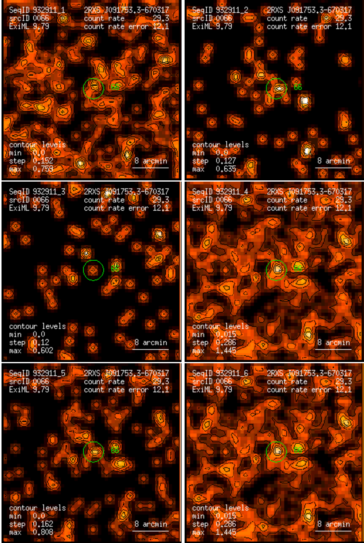
Figure 66: RASS 932911: detection 0066: band rate images, Gaussian filter: (1) PSPC channels 11 – 41, (2) 52 – 90, (3) 91 – 201, (4) 11 – 235, (5) 52 – 201, (6) 11 – 201. Broad band rates in counts/ks. Band rate contour levels in counts/ks/arcmin 2 .
