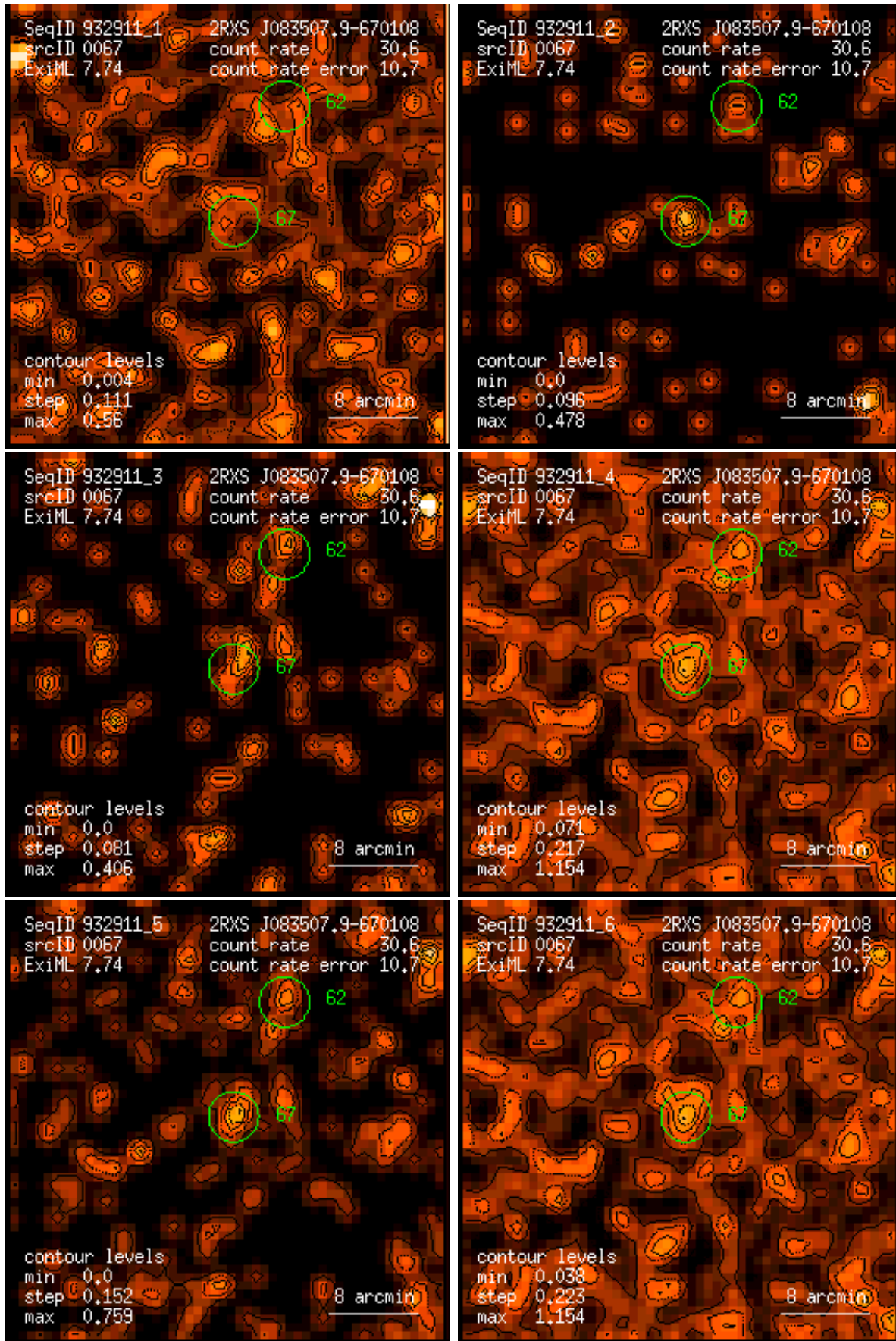
Figure 67: RASS 932911: detection 0067: band rate images, Gaussian filter: (1) PSPC channels 11 – 41, (2) 52 – 90, (3) 91 – 201, (4) 11 – 235, (5) 52 – 201, (6) 11 – 201. Broad band rates in counts/ks. Band rate contour levels in counts/ks/arcmin 2 .
