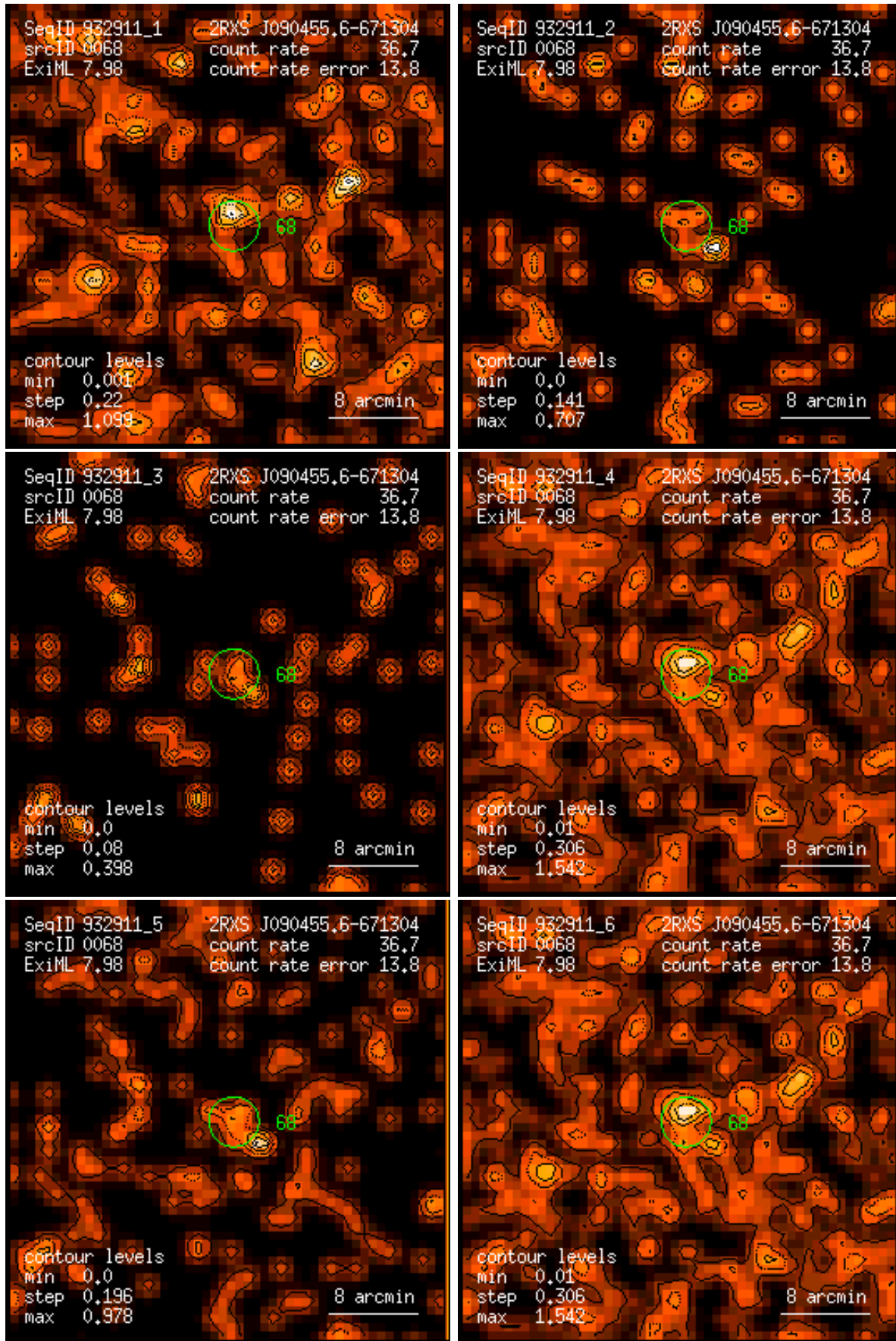
Figure 68: RASS 932911: detection 0068: band rate images, Gaussian filter: (1) PSPC channels 11 – 41, (2) 52 – 90, (3) 91 – 201, (4) 11 – 235, (5) 52 – 201, (6) 11 – 201. Broad band rates in counts/ks. Band rate contour levels in counts/ks/arcmin 2 .
