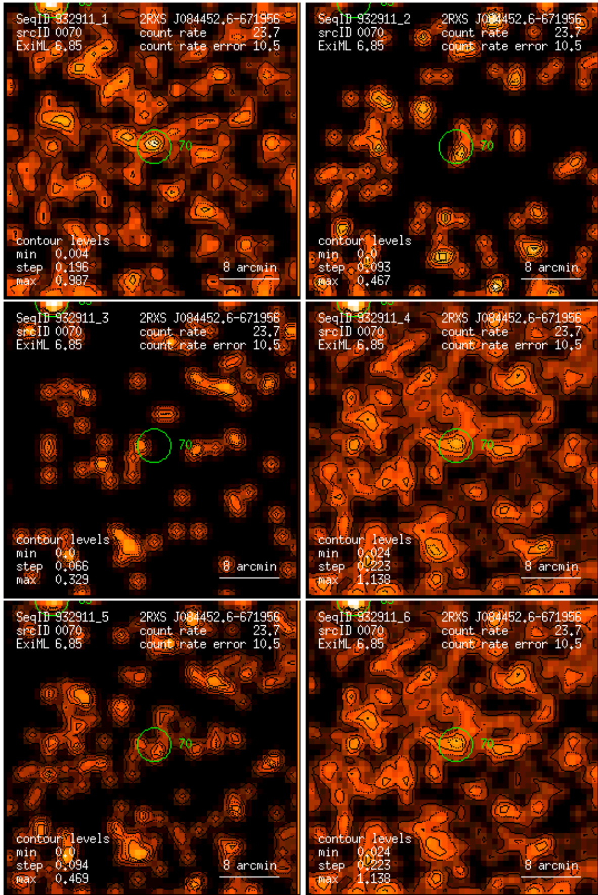
Figure 70: RASS 932911: detection 0070: band rate images, Gaussian filter: (1) PSPC channels 11 – 41, (2) 52 – 90, (3) 91 – 201, (4) 11 – 235, (5) 52 – 201, (6) 11 – 201. Broad band rates in counts/ks. Band rate contour levels in counts/ks/arcmin 2 .
