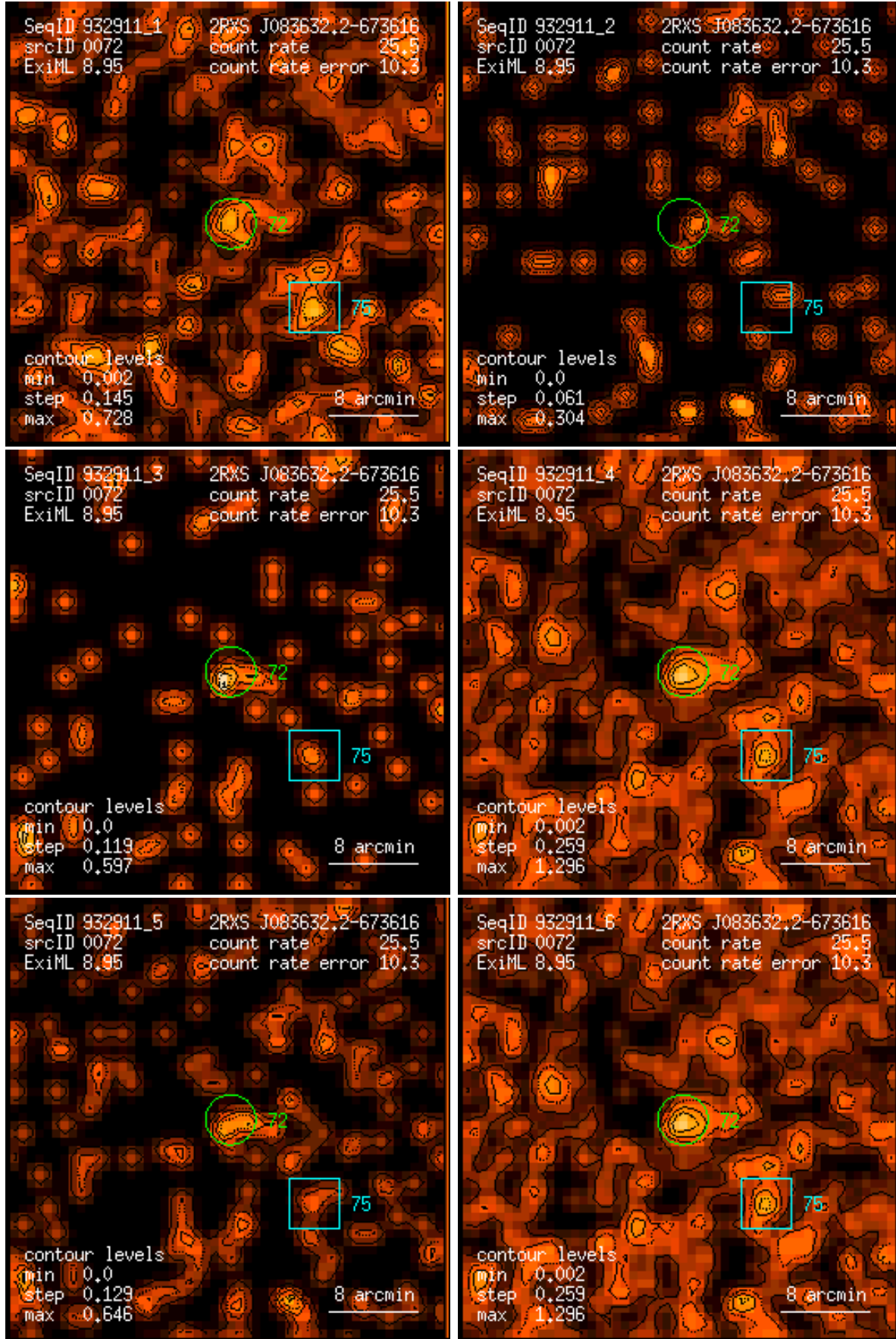
Figure 72: RASS 932911: detection 0072: band rate images, Gaussian filter: (1) PSPC channels 11 – 41, (2) 52 – 90, (3) 91 – 201, (4) 11 – 235, (5) 52 – 201, (6) 11 – 201. Broad band rates in counts/ks. Band rate contour levels in counts/ks/arcmin 2 .
