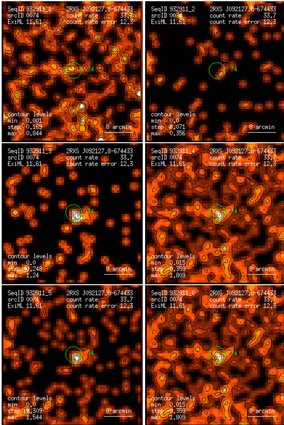
Figure 74: RASS 932911: detection 0074: band rate images, Gaussian filter: (1) PSPC channels 11 – 41, (2) 52 – 90, (3) 91 – 201, (4) 11 – 235, (5) 52 – 201, (6) 11 – 201. Broad band rates in counts/ks. Band rate contour levels in counts/ks/arcmin 2 .
