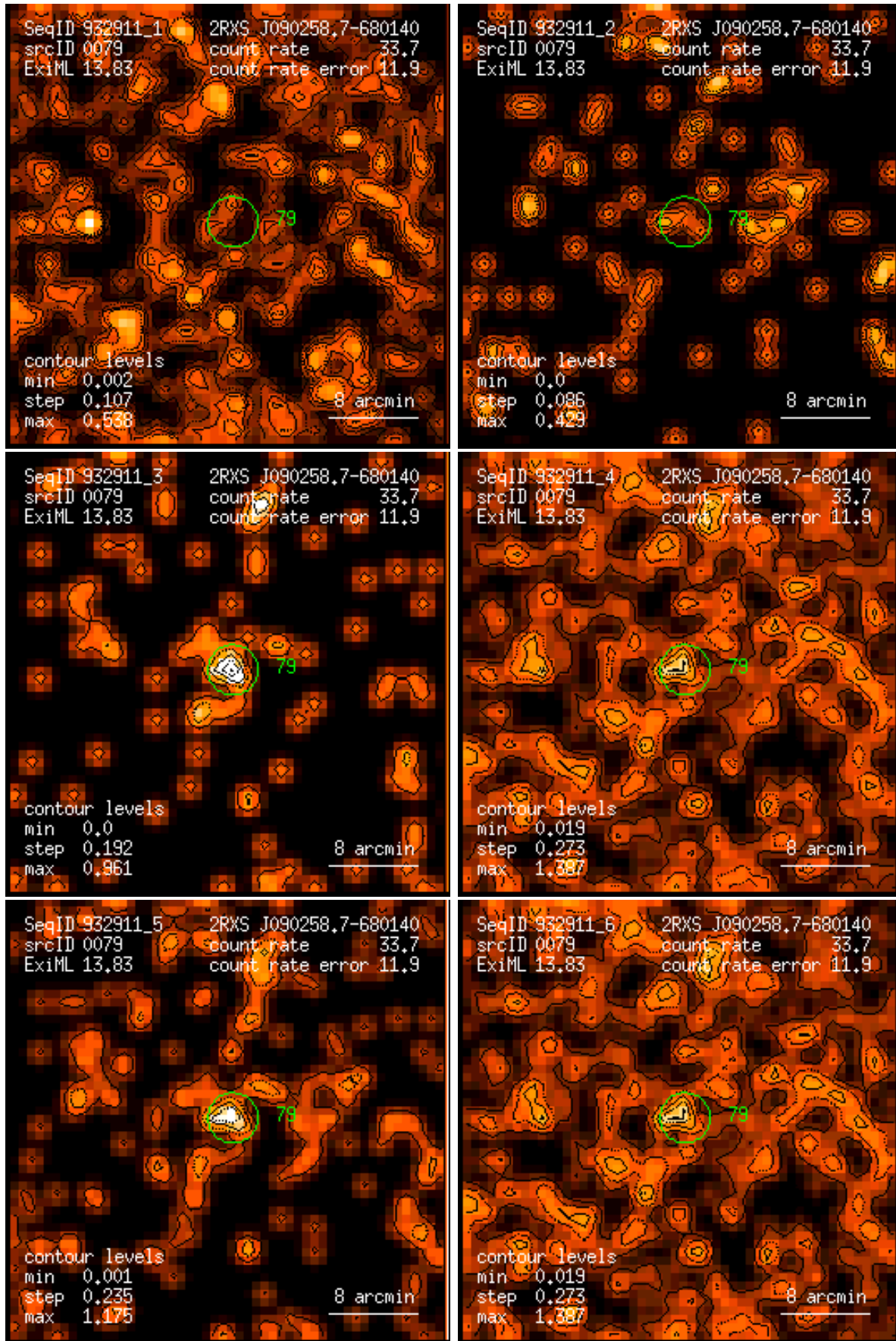
Figure 79: RASS 932911: detection 0079: band rate images, Gaussian filter: (1) PSPC channels 11 – 41, (2) 52 – 90, (3) 91 – 201, (4) 11 – 235, (5) 52 – 201, (6) 11 – 201. Broad band rates in counts/ks. Band rate contour levels in counts/ks/arcmin 2 .
