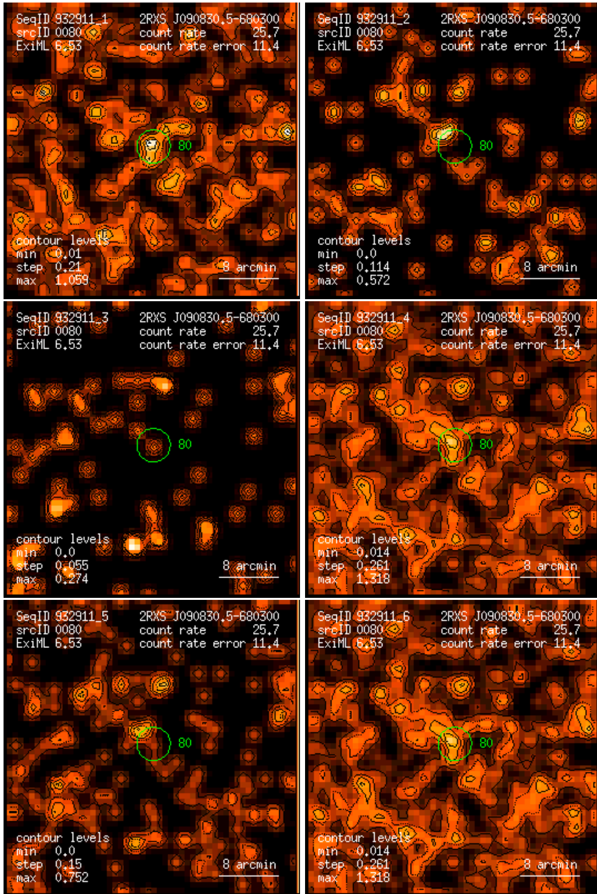
Figure 80: RASS 932911: detection 0080: band rate images, Gaussian filter: (1) PSPC channels 11 – 41, (2) 52 – 90, (3) 91 – 201, (4) 11 – 235, (5) 52 – 201, (6) 11 – 201. Broad band rates in counts/ks. Band rate contour levels in counts/ks/arcmin 2 .
