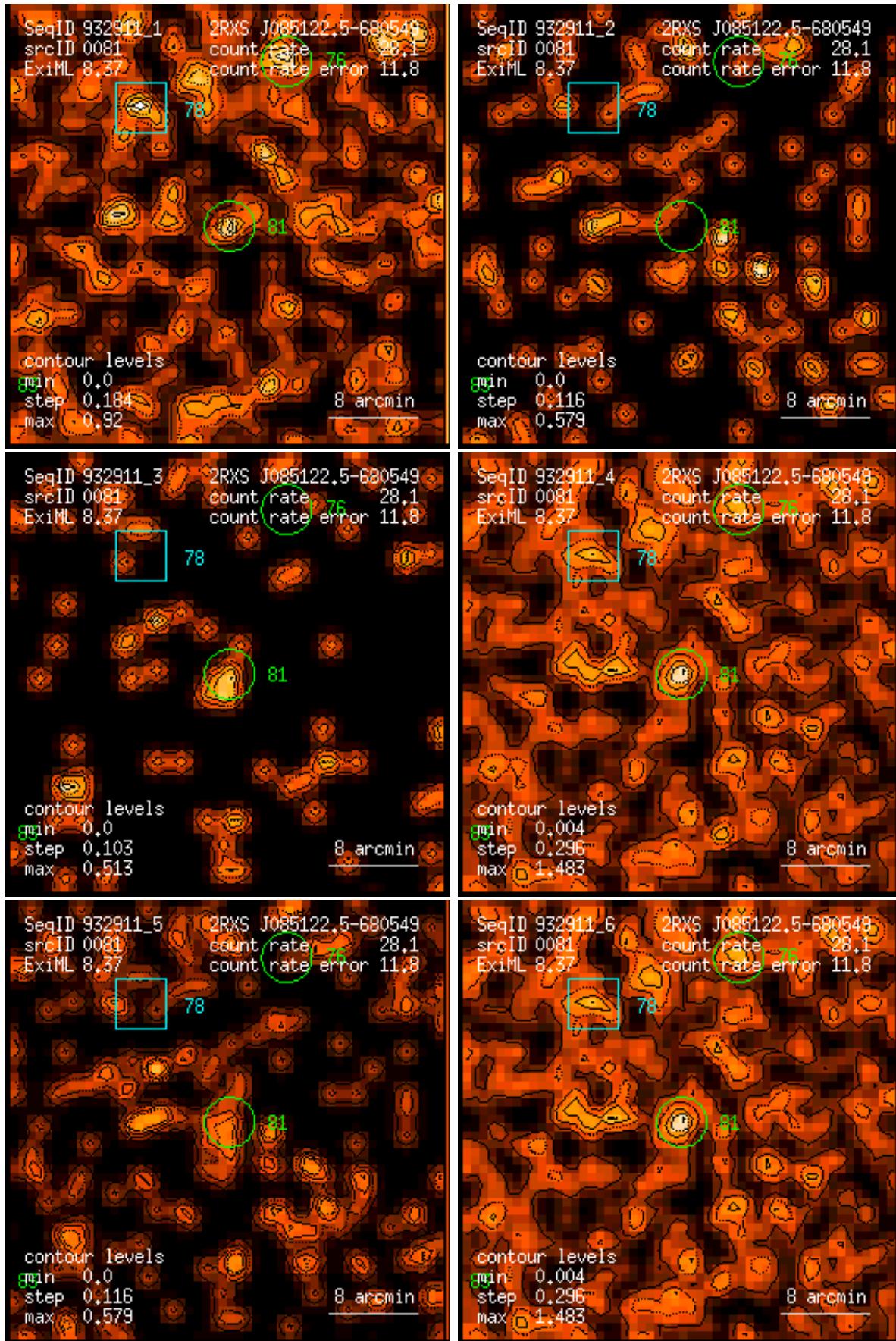
Figure 81: RASS 932911: detection 0081: band rate images, Gaussian filter: (1) PSPC channels 11 – 41, (2) 52 – 90, (3) 91 – 201, (4) 11 – 235, (5) 52 – 201, (6) 11 – 201. Broad band rates in counts/ks. Band rate contour levels in counts/ks/arcmin 2 .
