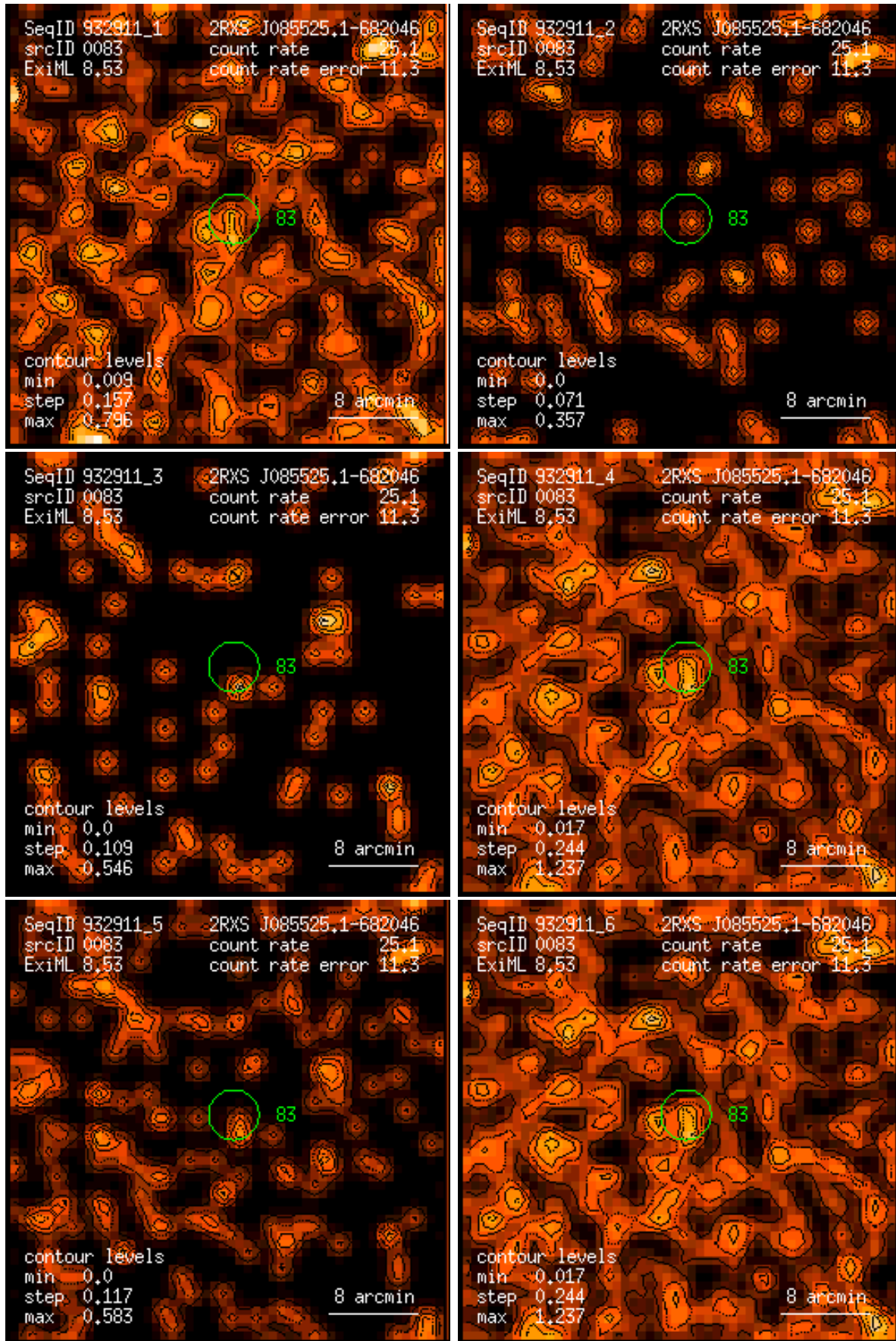
Figure 83: RASS 932911: detection 0083: band rate images, Gaussian filter: (1) PSPC channels 11 – 41, (2) 52 – 90, (3) 91 – 201, (4) 11 – 235, (5) 52 – 201, (6) 11 – 201. Broad band rates in counts/ks. Band rate contour levels in counts/ks/arcmin 2 .
