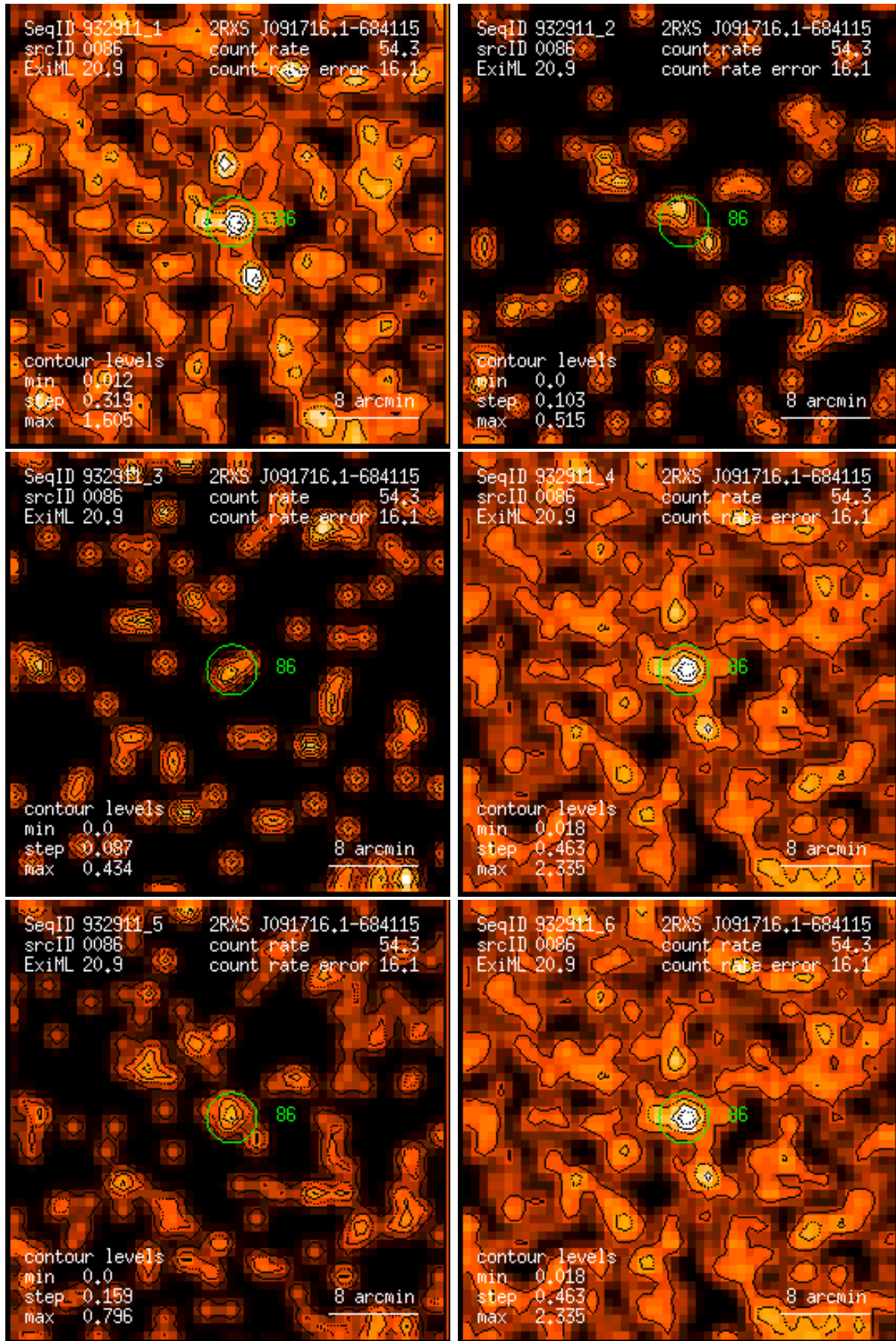
Figure 86: RASS 932911: detection 0086: band rate images, Gaussian filter: (1) PSPC channels 11 – 41, (2) 52 – 90, (3) 91 – 201, (4) 11 – 235, (5) 52 – 201, (6) 11 – 201. Broad band rates in counts/ks. Band rate contour levels in counts/ks/arcmin 2 .
