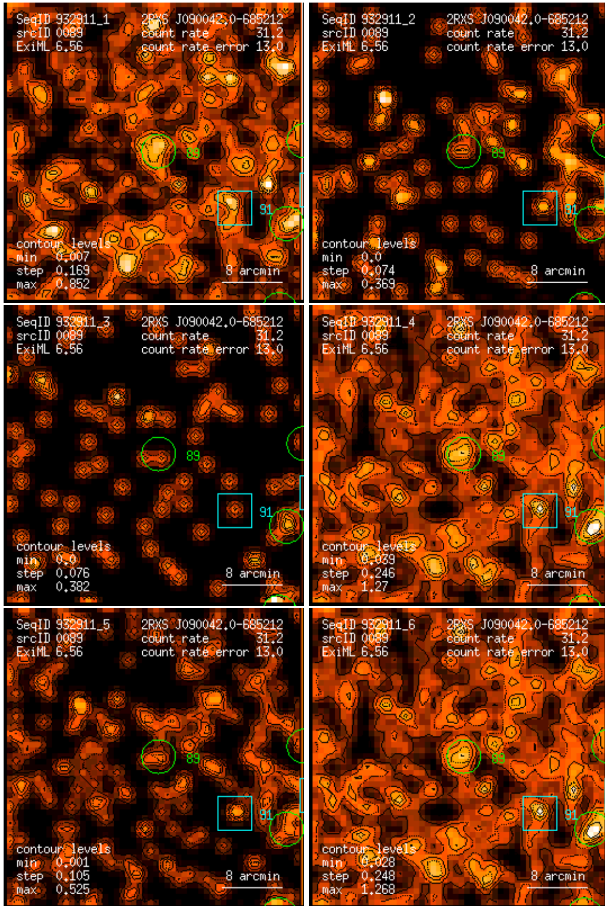
Figure 89: RASS 932911: detection 0089: band rate images, Gaussian filter: (1) PSPC channels 11 – 41, (2) 52 – 90, (3) 91 – 201, (4) 11 – 235, (5) 52 – 201, (6) 11 – 201. Broad band rates in counts/ks. Band rate contour levels in counts/ks/arcmin 2 .
