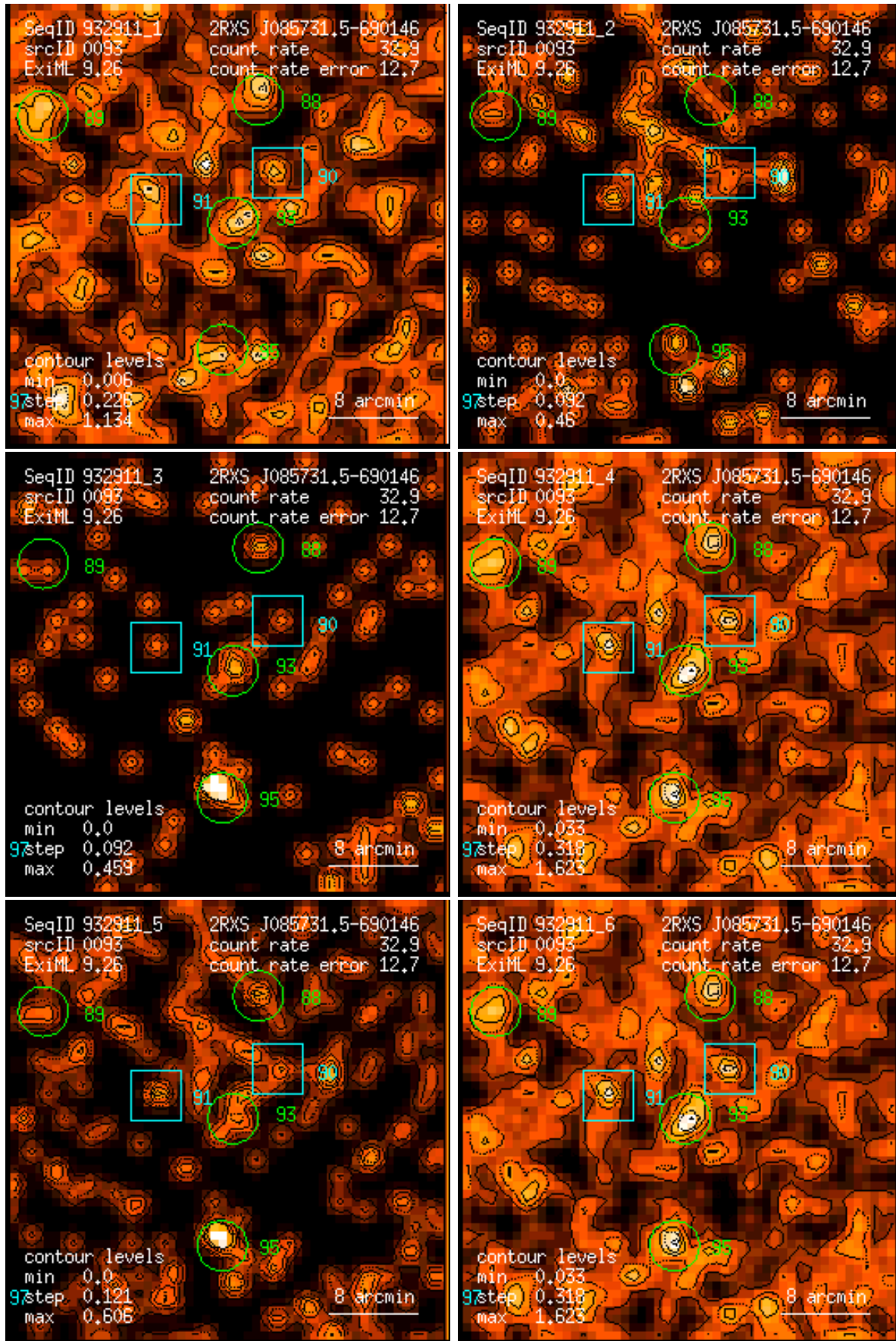
Figure 93: RASS 932911: detection 0093: band rate images, Gaussian filter: (1) PSPC channels 11 – 41, (2) 52 – 90, (3) 91 – 201, (4) 11 – 235, (5) 52 – 201, (6) 11 – 201. Broad band rates in counts/ks. Band rate contour levels in counts/ks/arcmin 2 .
