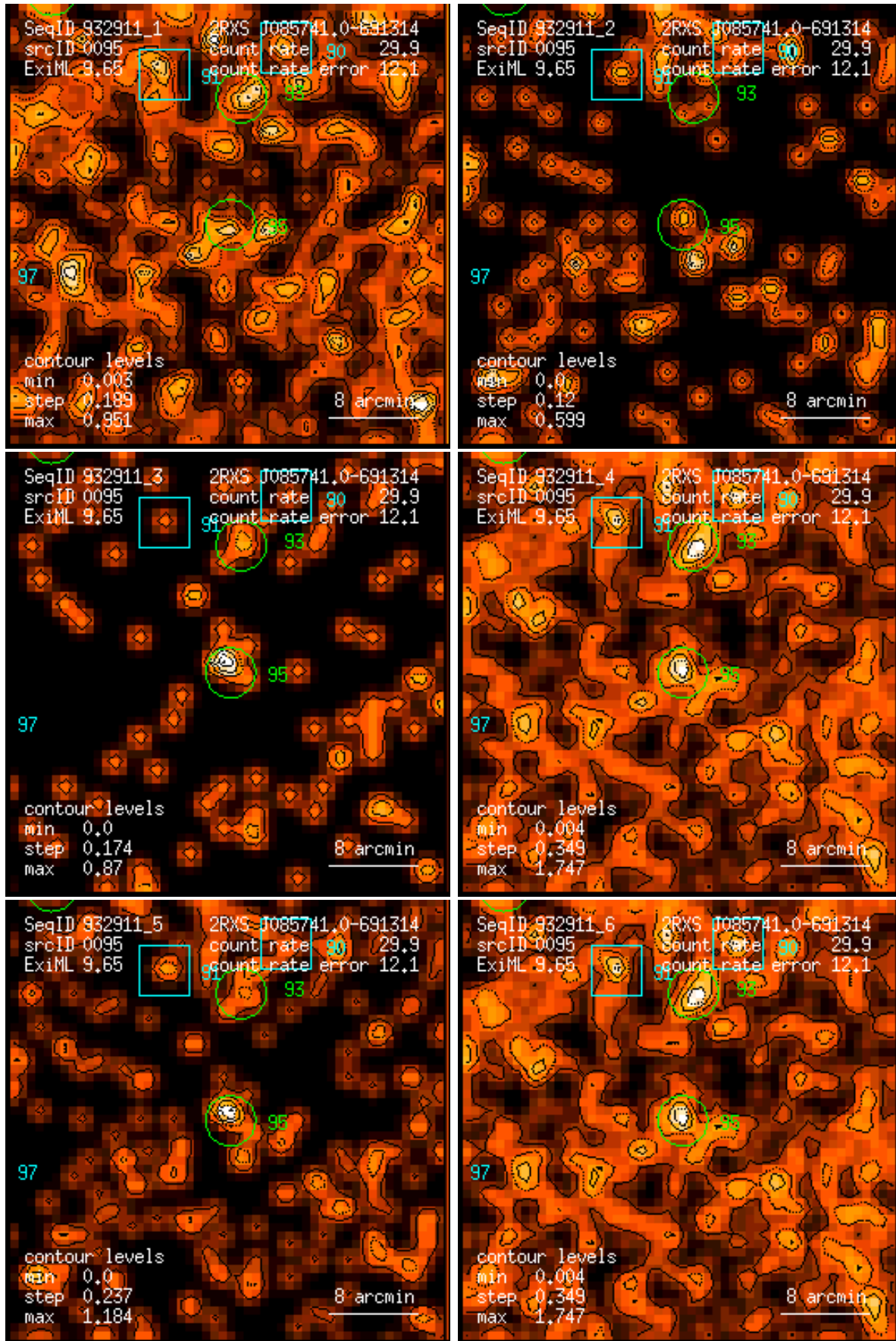
Figure 95: RASS 932911: detection 0095: band rate images, Gaussian filter: (1) PSPC channels 11 – 41, (2) 52 – 90, (3) 91 – 201, (4) 11 – 235, (5) 52 – 201, (6) 11 – 201. Broad band rates in counts/ks. Band rate contour levels in counts/ks/arcmin 2 .
