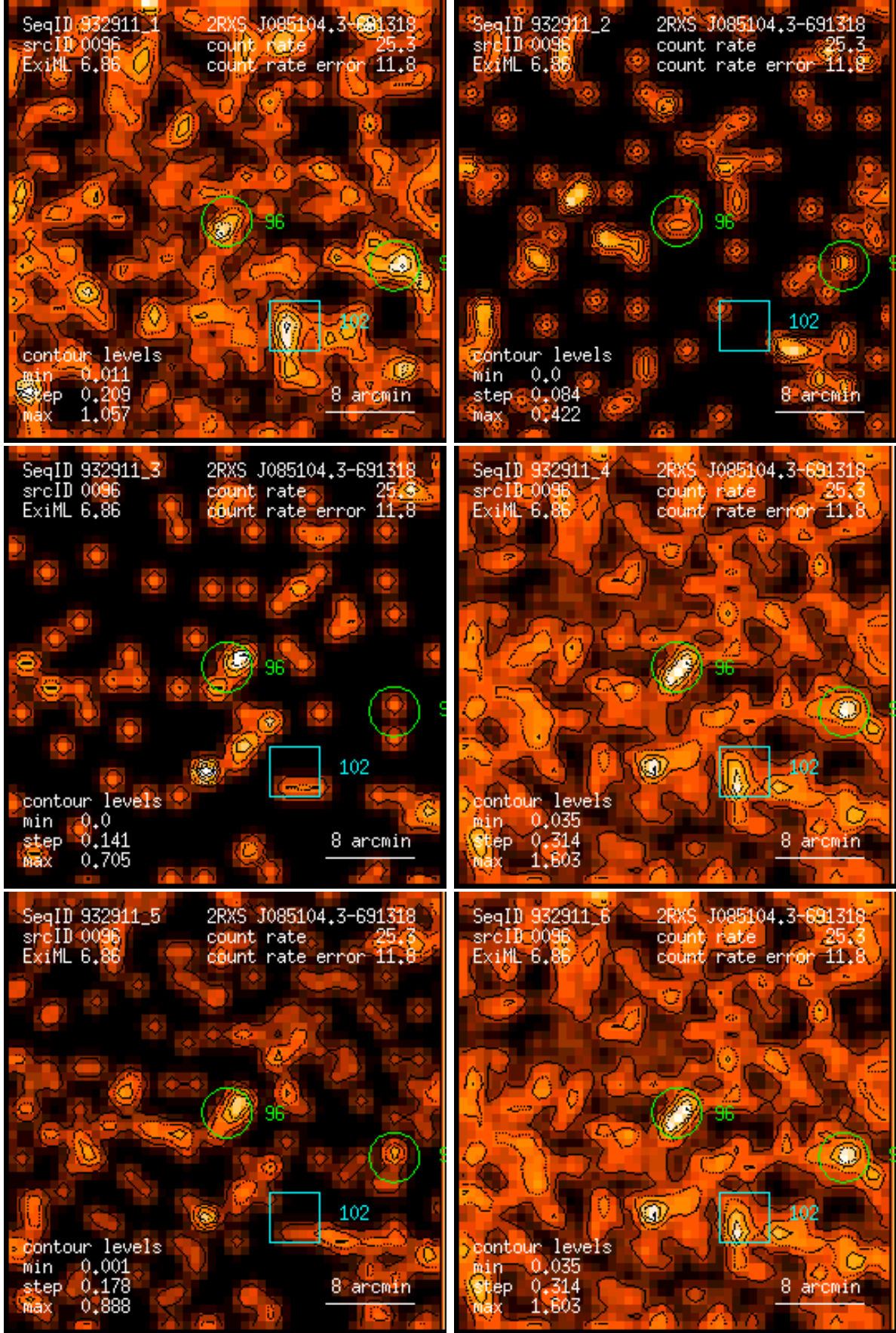
Figure 96: RASS 932911: detection 0096: band rate images, Gaussian filter: (1) PSPC channels 11 – 41, (2) 52 – 90, (3) 91 – 201, (4) 11 – 235, (5) 52 – 201, (6) 11 – 201. Broad band rates in counts/ks. Band rate contour levels in counts/ks/arcmin 2 .
