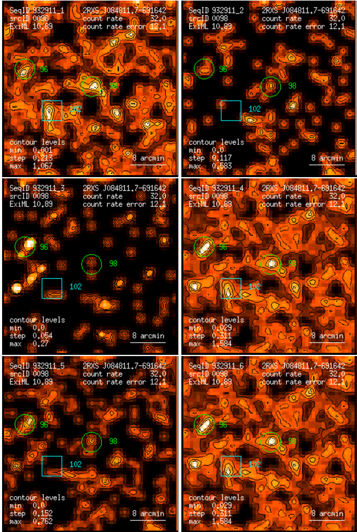
Figure 98: RASS 932911: detection 0098: band rate images, Gaussian filter: (1) PSPC channels 11 – 41, (2) 52 – 90, (3) 91 – 201, (4) 11 – 235, (5) 52 – 201, (6) 11 – 201. Broad band rates in counts/ks. Band rate contour levels in counts/ks/arcmin 2 .
