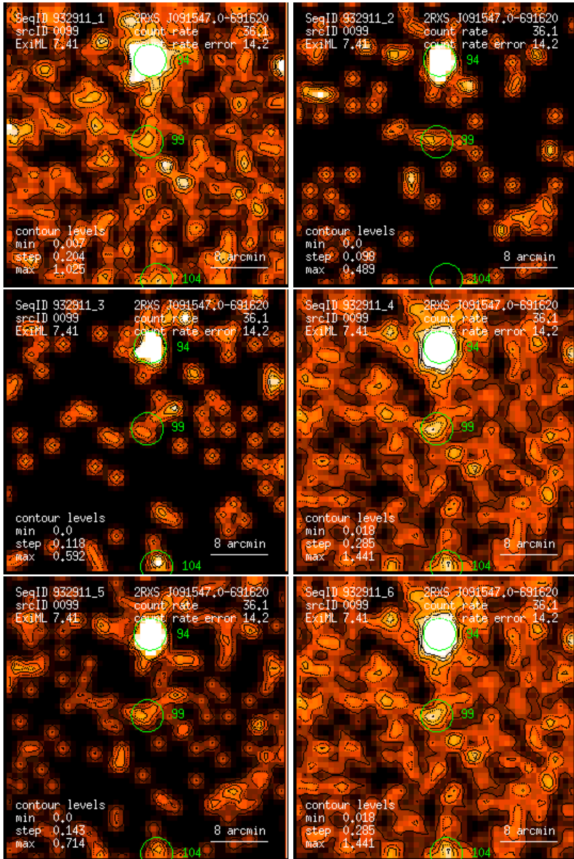
Figure 99: RASS 932911: detection 0099: band rate images, Gaussian filter: (1) PSPC channels 11 – 41, (2) 52 – 90, (3) 91 – 201, (4) 11 – 235, (5) 52 – 201, (6) 11 – 201. Broad band rates in counts/ks. Band rate contour levels in counts/ks/arcmin 2 .
