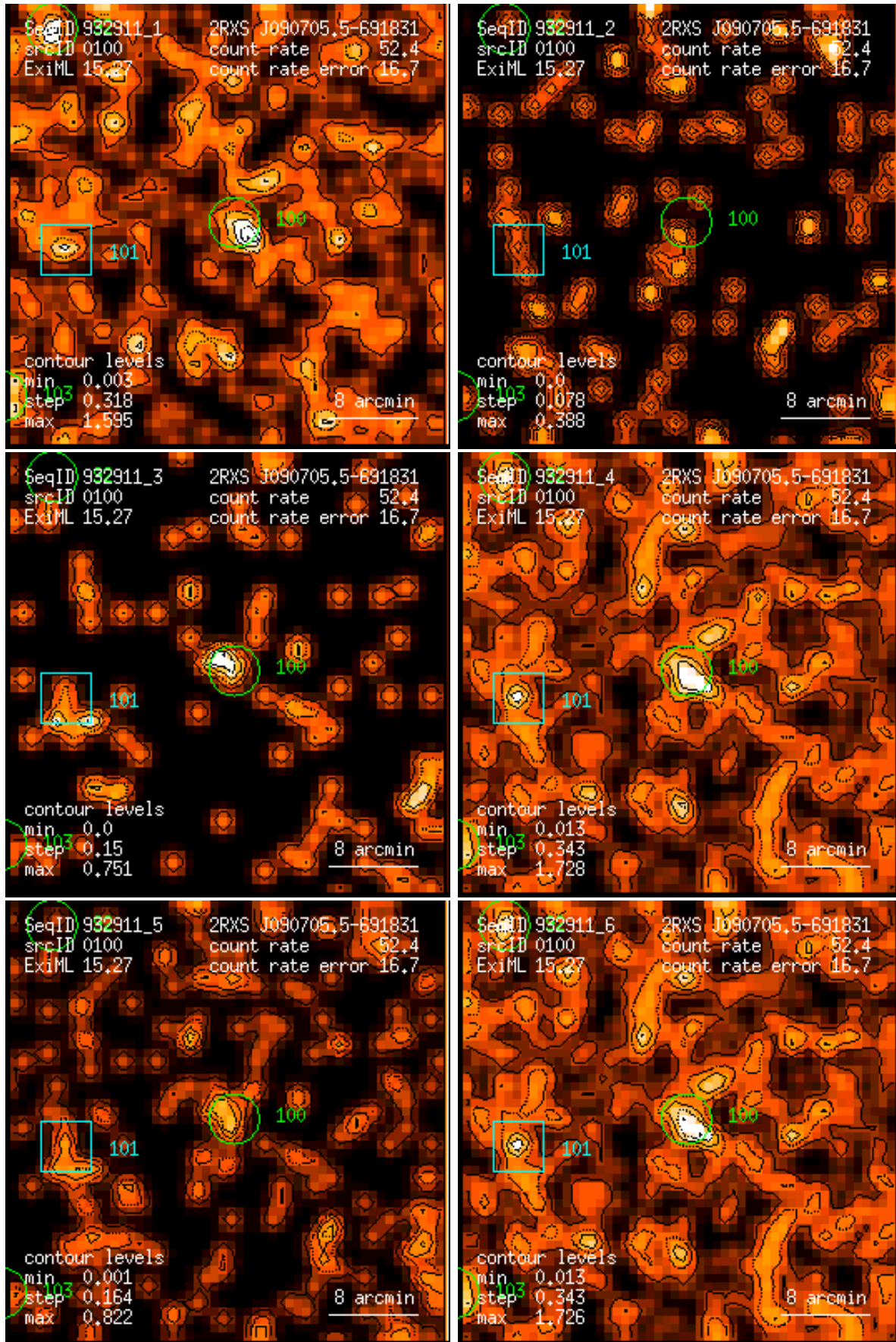
Figure 100: RASS 932911: detection 0100: band rate images, Gaussian filter: (1) PSPC channels 11 – 41, (2) 52 – 90, (3) 91 – 201, (4) 11 – 235, (5) 52 – 201, (6) 11 – 201. Broad band rates in counts/ks. Band rate contour levels in counts/ks/arcmin 2 .
