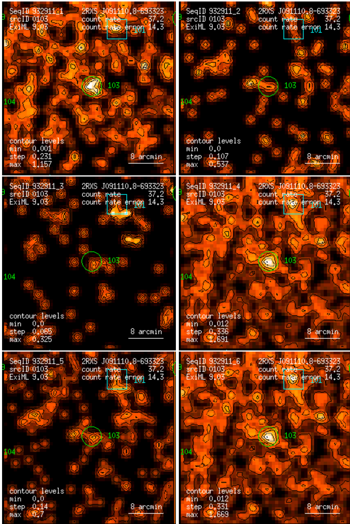
Figure 103: RASS 932911: detection 0103: band rate images, Gaussian filter: (1) PSPC channels 11 – 41, (2) 52 – 90, (3) 91 – 201, (4) 11 – 235, (5) 52 – 201, (6) 11 – 201. Broad band rates in counts/ks. Band rate contour levels in counts/ks/arcmin 2 .
