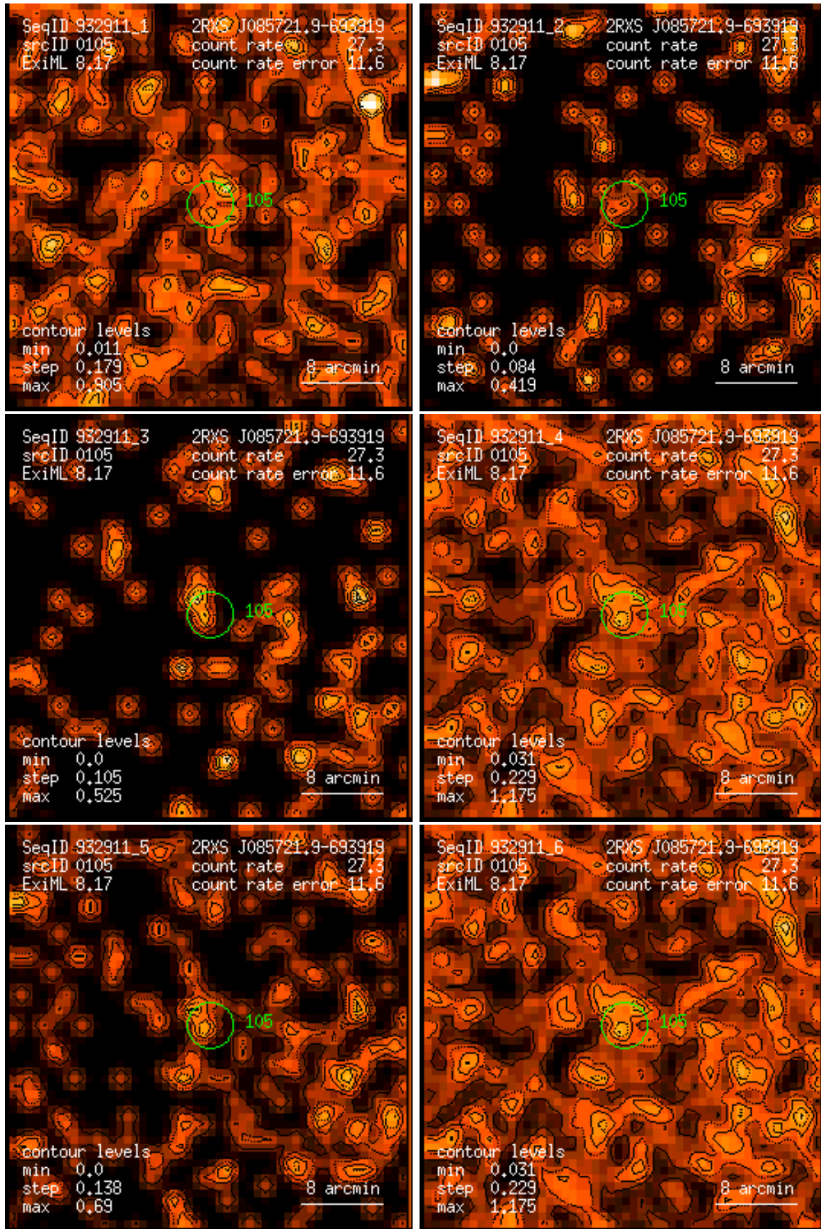
Figure 105: RASS 932911: detection 0105: band rate images, Gaussian filter: (1) PSPC channels 11 – 41, (2) 52 – 90, (3) 91 – 201, (4) 11 – 235, (5) 52 – 201, (6) 11 – 201. Broad band rates in counts/ks. Band rate contour levels in counts/ks/arcmin 2 .
