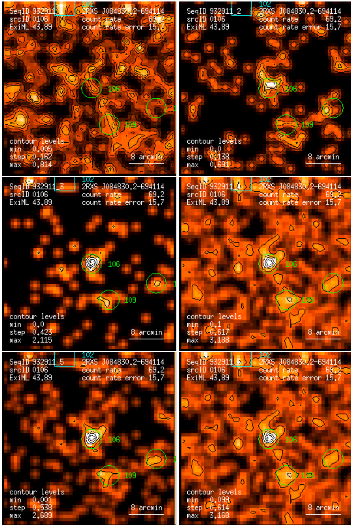
Figure 106: RASS 932911: detection 0106: band rate images, Gaussian filter: (1) PSPC channels 11 – 41, (2) 52 – 90, (3) 91 – 201, (4) 11 – 235, (5) 52 – 201, (6) 11 – 201. Broad band rates in counts/ks. Band rate contour levels in counts/ks/arcmin 2 .
