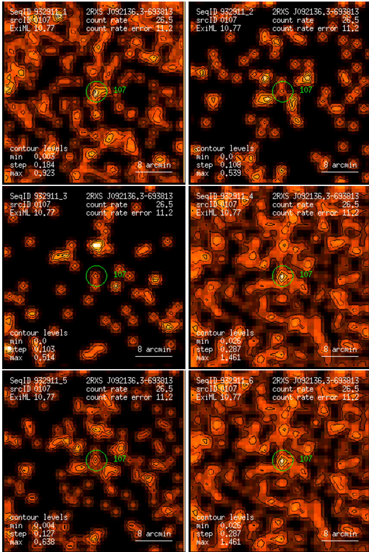
Figure 107: RASS 932911: detection 0107: band rate images, Gaussian filter: (1) PSPC channels 11 – 41, (2) 52 – 90, (3) 91 – 201, (4) 11 – 235, (5) 52 – 201, (6) 11 – 201. Broad band rates in counts/ks. Band rate contour levels in counts/ks/arcmin 2 .
