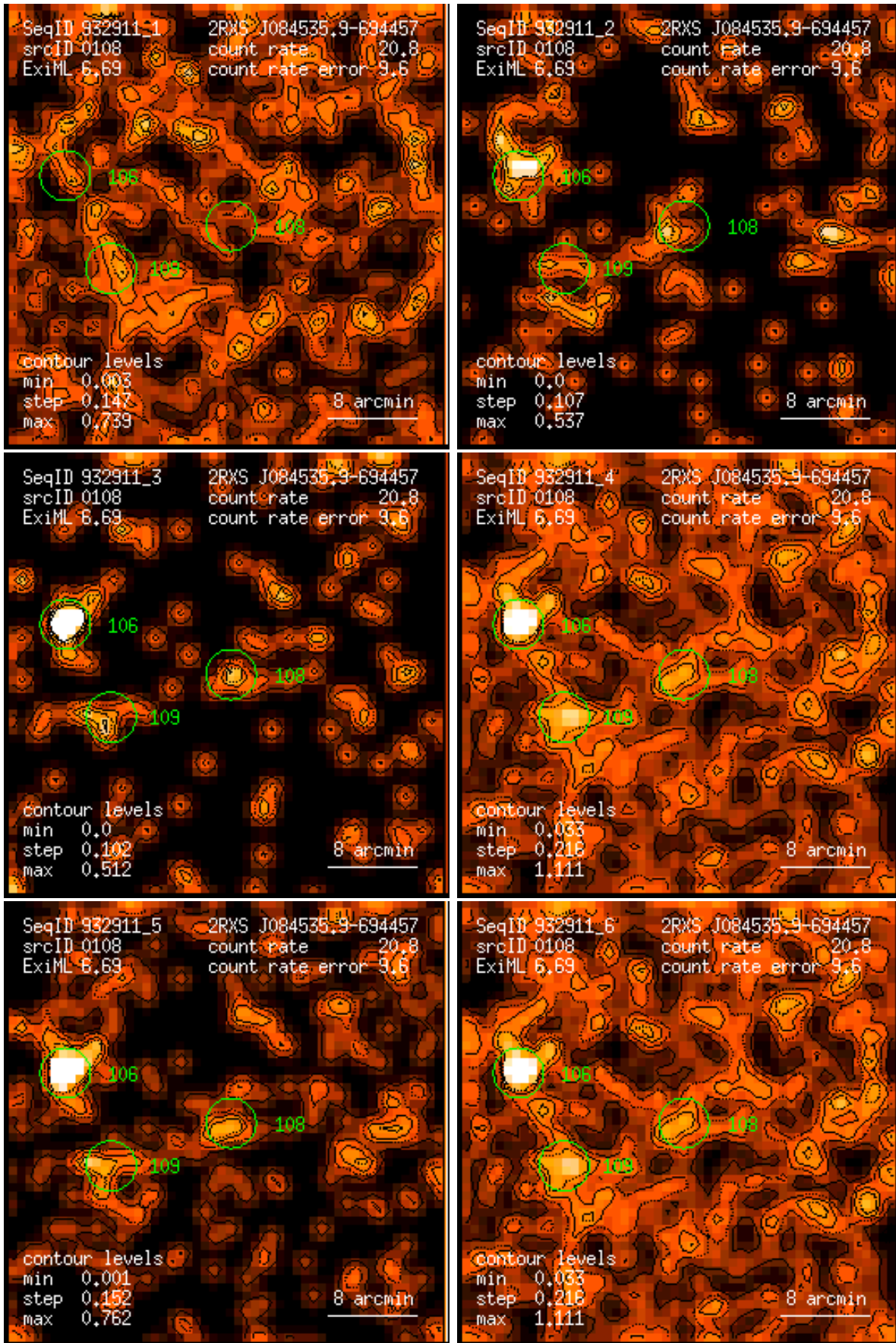
Figure 108: RASS 932911: detection 0108: band rate images, Gaussian filter: (1) PSPC channels 11 – 41, (2) 52 – 90, (3) 91 – 201, (4) 11 – 235, (5) 52 – 201, (6) 11 – 201. Broad band rates in counts/ks. Band rate contour levels in counts/ks/arcmin 2 .
