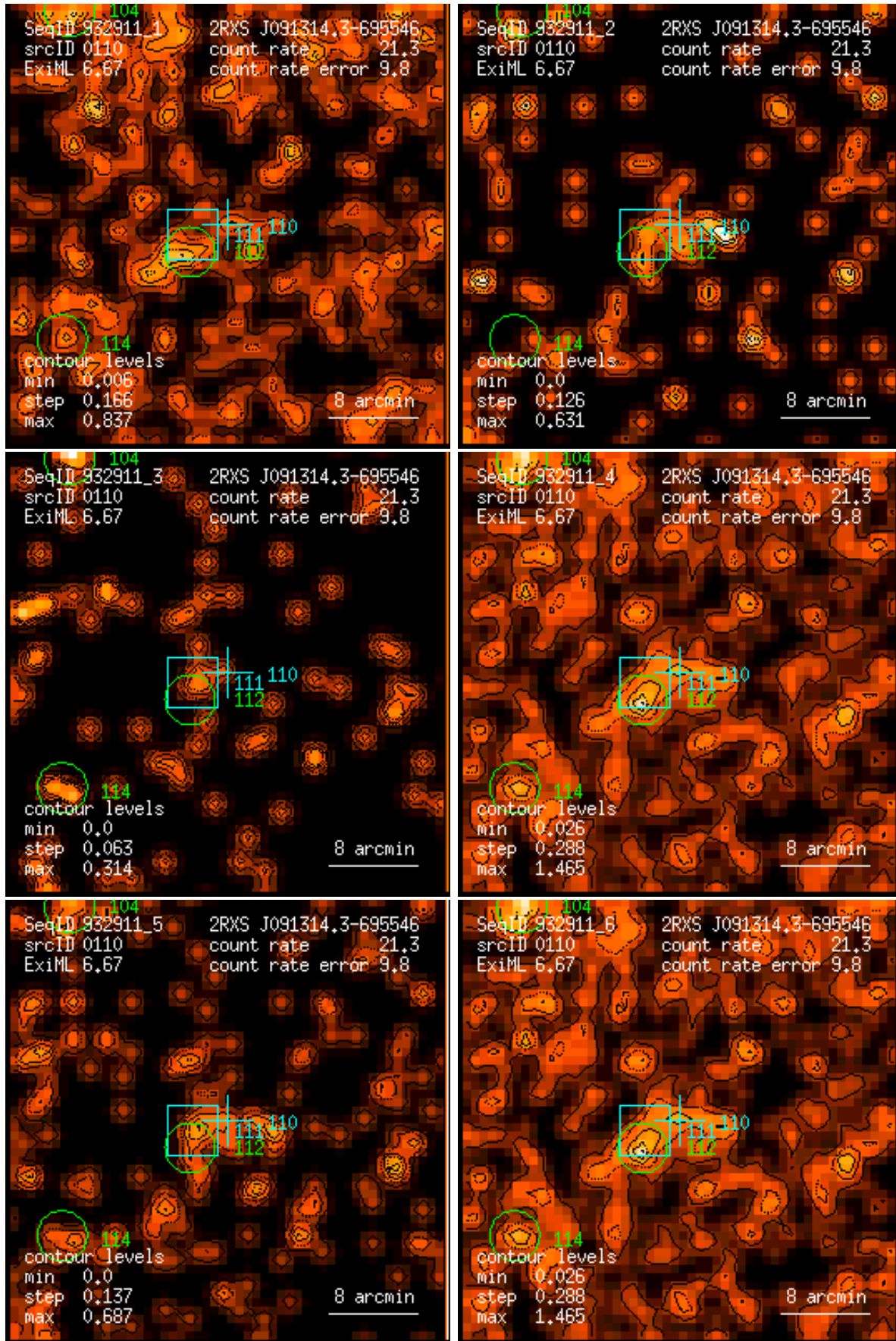
Figure 110: RASS 932911: detection 0110: band rate images, Gaussian filter: (1) PSPC channels 11 – 41, (2) 52 – 90, (3) 91 – 201, (4) 11 – 235, (5) 52 – 201, (6) 11 – 201. Broad band rates in counts/ks. Band rate contour levels in counts/ks/arcmin 2 .
